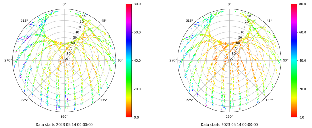
Skyplot for station RIO1. Parameter M1C Data file RIO100ESP_R_2023134.xtr Skyplot for station RIO1. Parameter M2P Data file RIO100ESP_R_2023134.xtr
