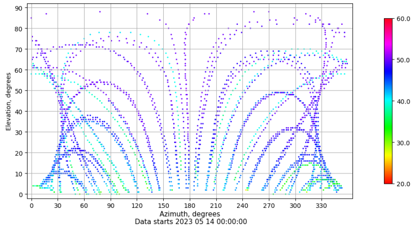
Azimuth-elevation plot for station RIO1. Signal to Noise S1C Data file RIO100ESP_R_2023134.xtr
