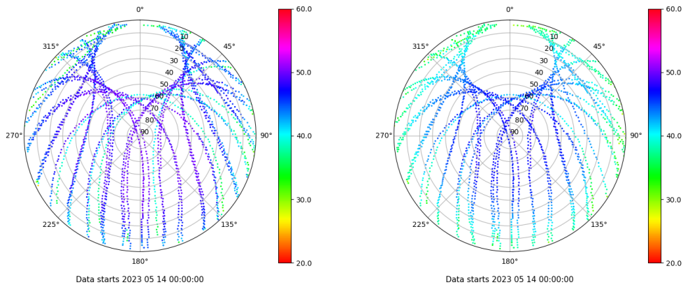
Skyplot for station RIO1. Signal to Noise S1C Data file RIO100ESP_R_2023134.xtr Skyplot for station RIO1. Signal to Noise S2P Data file RIO100ESP_R_2023134.xtr
