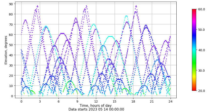
Time-elevation plot for station RIO1. Signal to Noise S1C Data file RIO100ESP_R_2023134.xtr
