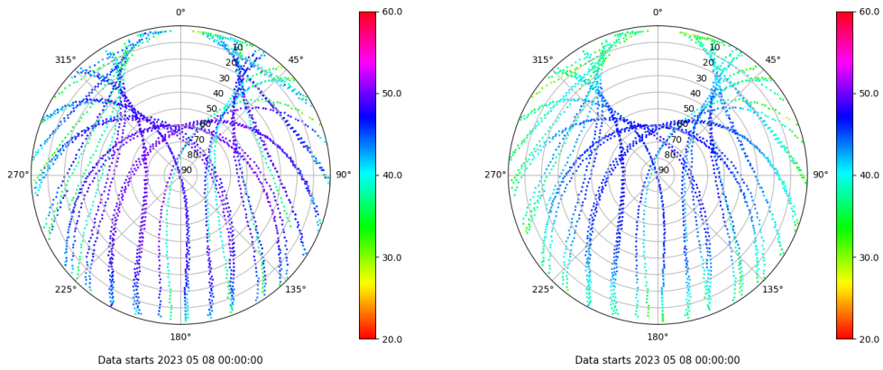
Skyplot for station RIO1. Signal to Noise S1C Data file RIO100ESP_R_2023128.xtr Skyplot for station RIO1. Signal to Noise S2P Data file RIO100ESP_R_2023128.xtr
