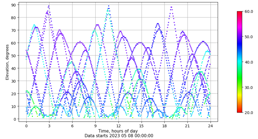
Time-elevation plot for station RIO1. Signal to Noise S1C Data file RIO100ESP_R_2023128.xtr
