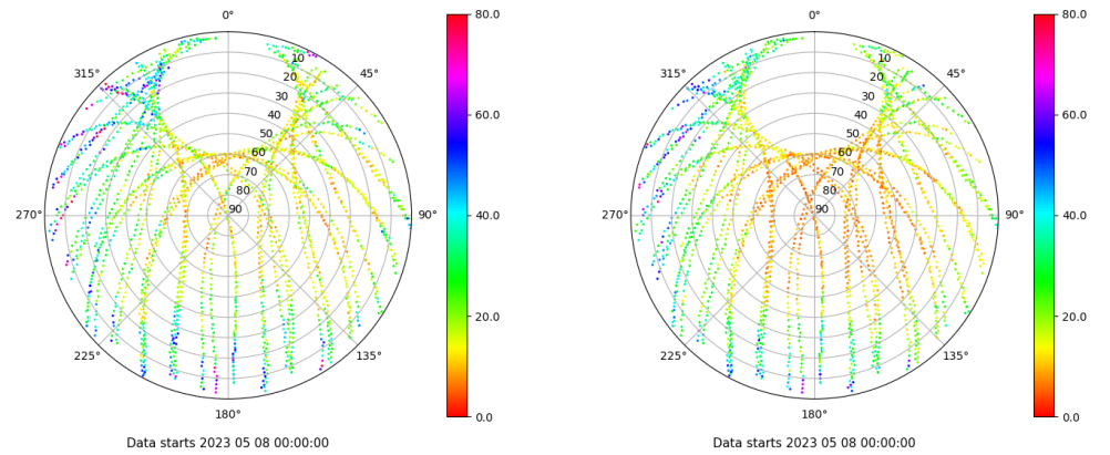
Skyplot for station RIO1. Parameter M1C Data file RIO100ESP_R_2023128.xtr Skyplot for station RIO1. Parameter M2P Data file RIO100ESP_R_2023128.xtr
