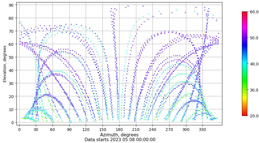
Azimuth-elevation plot for station RIO1. Signal to Noise S1C Data file RIO100ESP_R_2023128.xtr
