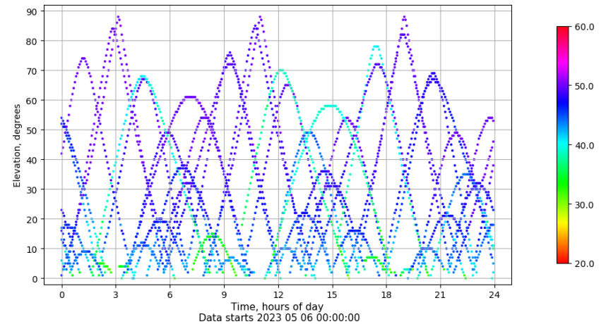
Time-elevation plot for station RIO1. Signal to Noise S1C Data file RIO100ESP_R_2023126.xtr
