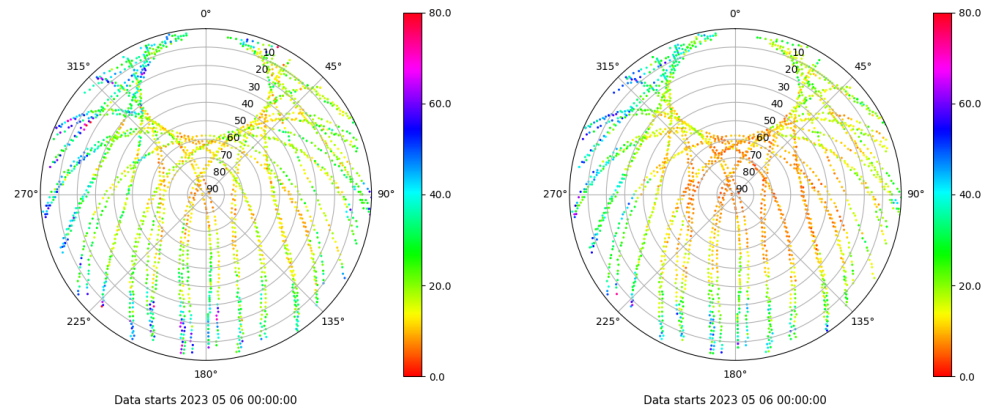
Skyplot for station RIO1. Parameter M1C Data file RIO100ESP_R_2023126.xtr Skyplot for station RIO1. Parameter M2P Data file RIO100ESP_R_2023126.xtr
