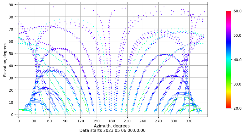
Azimuth-elevation plot for station RIO1. Signal to Noise S1C Data file RIO100ESP_R_2023126.xtr
