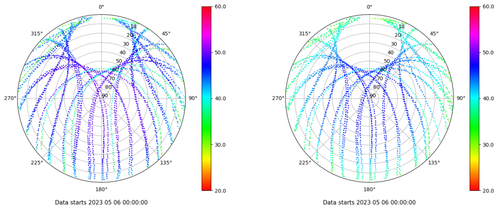
Skyplot for station RIO1. Signal to Noise S1C Data file RIO100ESP_R_2023126.xtr Skyplot for station RIO1. Signal to Noise S2P Data file RIO100ESP_R_2023126.xtr
