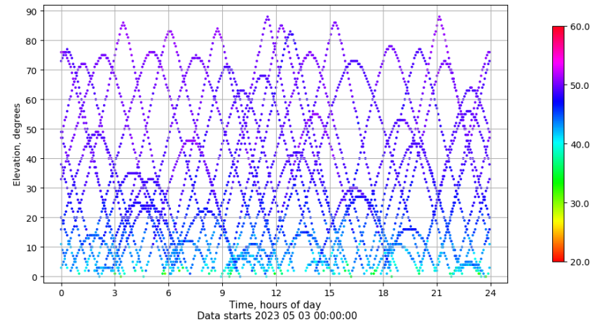
Time-elevation plot for station RIO1. Signal to Noise S1C Data file RIO100ESP_R_2023123.xtr
