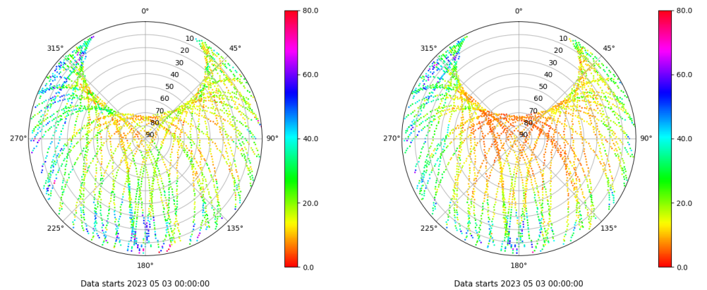
Skyplot for station RIO1. Parameter M1C Data file RIO100ESP_R_2023123.xtr Skyplot for station RIO1. Parameter M2W Data file RIO100ESP_R_2023123.xtr
