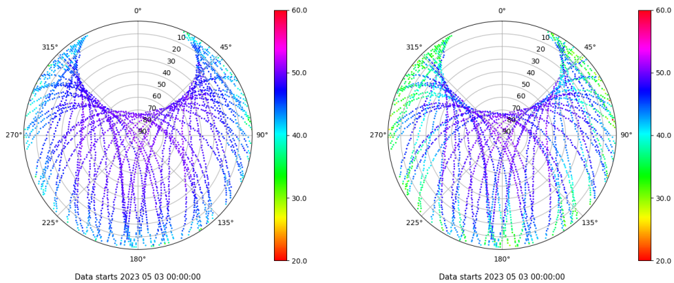
Skyplot for station RIO1. Signal to Noise S1C Data file RIO100ESP_R_2023123.xtr Skyplot for station RIO1. Signal to Noise S2W Data file RIO100ESP_R_2023123.xtr
