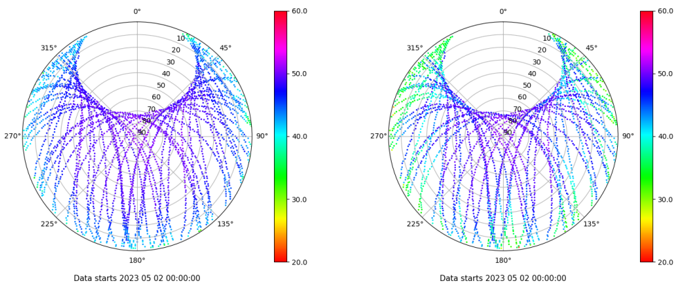
Skyplot for station RIO1. Signal to Noise S1C Data file RIO100ESP_R_2023122.xtr Skyplot for station RIO1. Signal to Noise S2W Data file RIO100ESP_R_2023122.xtr
