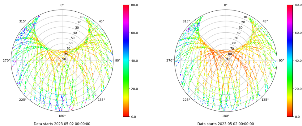
Skyplot for station RIO1. Parameter M1C Data file RIO100ESP_R_2023122.xtr Skyplot for station RIO1. Parameter M2W Data file RIO100ESP_R_2023122.xtr
