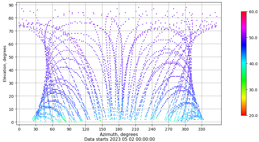
Azimuth-elevation plot for station RIO1. Signal to Noise S1C Data file RIO100ESP_R_2023122.xtr
