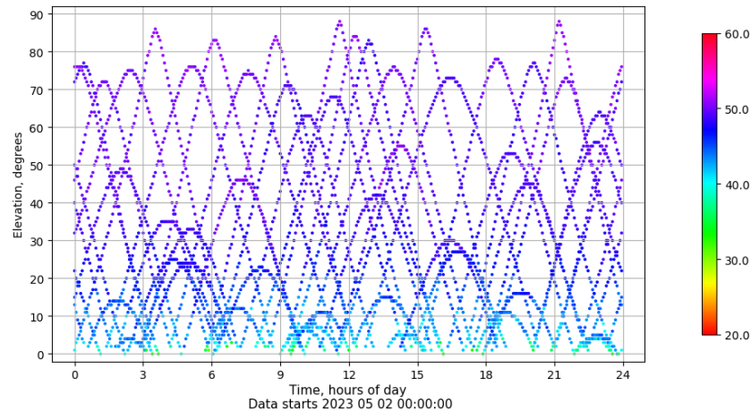
Time-elevation plot for station RIO1. Signal to Noise S1C Data file RIO100ESP_R_2023122.xtr
