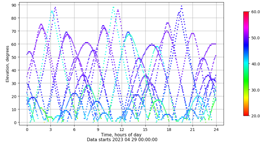
Time-elevation plot for station RIO1. Signal to Noise S1C Data file RIO100ESP_R_2023119.xtr
