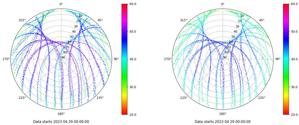
Skyplot for station RIO1. Signal to Noise S1C Data file RIO100ESP_R_2023119.xtr Skyplot for station RIO1. Signal to Noise S2P Data file RIO100ESP_R_2023119.xtr
