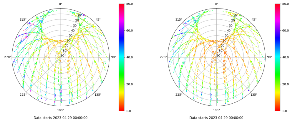
Skyplot for station RIO1. Parameter M1C Data file RIO100ESP_R_2023119.xtr Skyplot for station RIO1. Parameter M2P Data file RIO100ESP_R_2023119.xtr
