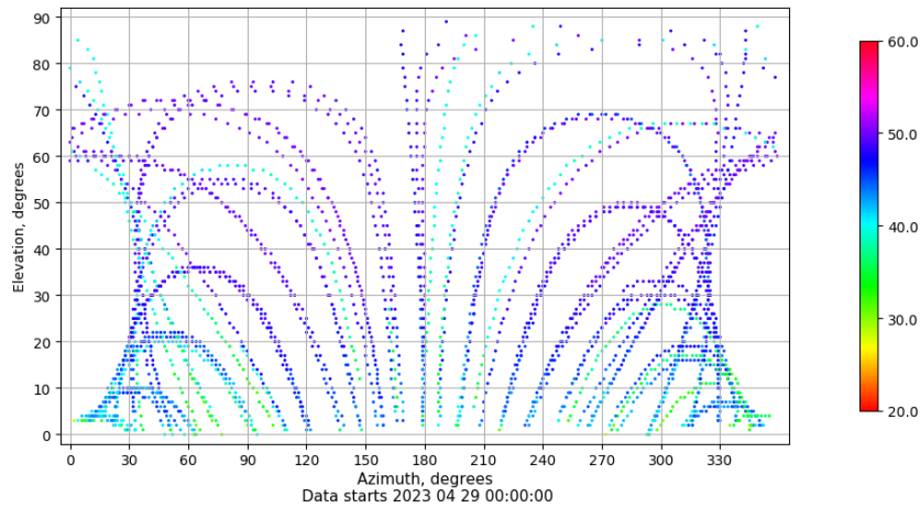
Azimuth-elevation plot for station RIO1. Signal to Noise S1C Data file RIO100ESP_R_2023119.xtr
