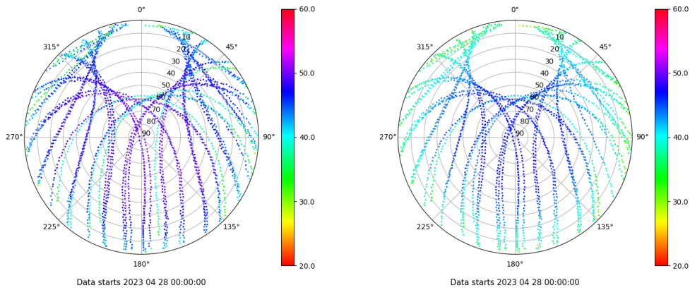
Skyplot for station RIO1. Signal to Noise S1C Data file RIO100ESP_R_2023118.xtr Skyplot for station RIO1. Signal to Noise S2P Data file RIO100ESP_R_2023118.xtr
