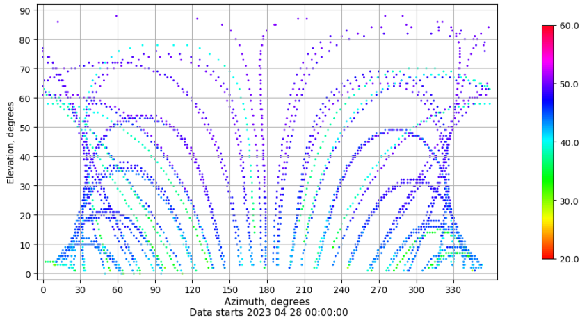
Azimuth-elevation plot for station RIO1. Signal to Noise S1C Data file RIO100ESP_R_2023118.xtr
