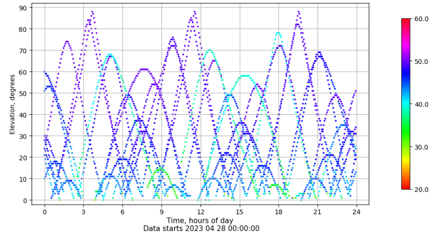
Time-elevation plot for station RIO1. Signal to Noise S1C Data file RIO100ESP_R_2023118.xtr
