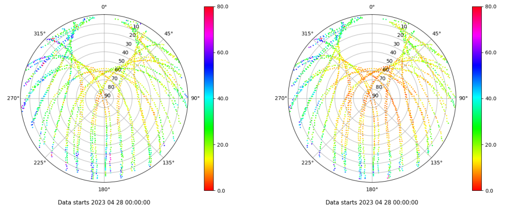
Skyplot for station RIO1. Parameter M1C Data file RIO100ESP_R_2023118.xtr Skyplot for station RIO1. Parameter M2P Data file RIO100ESP_R_2023118.xtr
