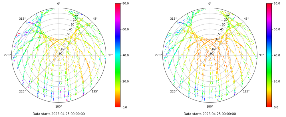
Skyplot for station RIO1. Parameter M1C Data file RIO100ESP_R_2023115.xtr Skyplot for station RIO1. Parameter M2P Data file RIO100ESP_R_2023115.xtr
