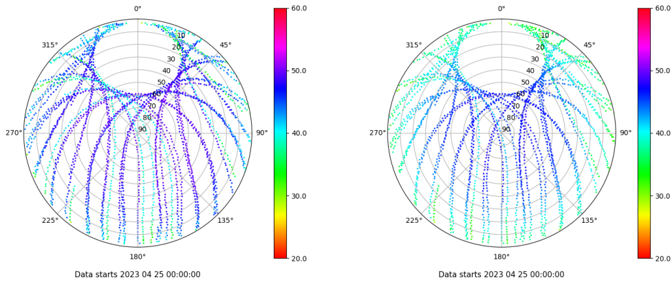
Skyplot for station RIO1. Signal to Noise S1C Data file RIO100ESP_R_2023115.xtr Skyplot for station RIO1. Signal to Noise S2P Data file RIO100ESP_R_2023115.xtr
