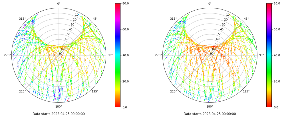
Skyplot for station RIO1. Parameter M1C Data file RIO100ESP_R_2023115.xtr Skyplot for station RIO1. Parameter M2W Data file RIO100ESP_R_2023115.xtr
