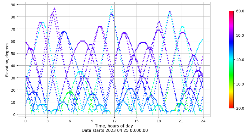
Time-elevation plot for station RIO1. Signal to Noise S1C Data file RIO100ESP_R_2023115.xtr
