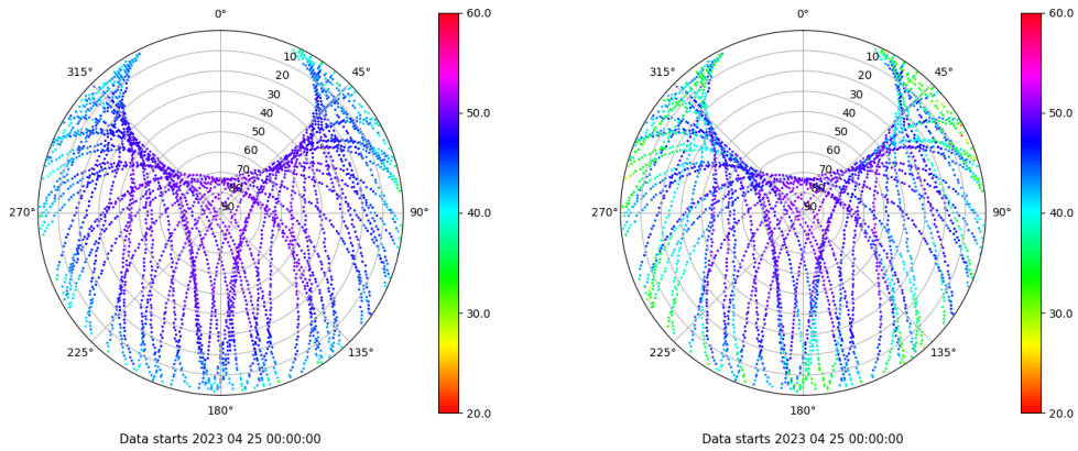
Skyplot for station RIO1. Signal to Noise S1C Data file RIO100ESP_R_2023115.xtr Skyplot for station RIO1. Signal to Noise S2W Data file RIO100ESP_R_2023115.xtr
