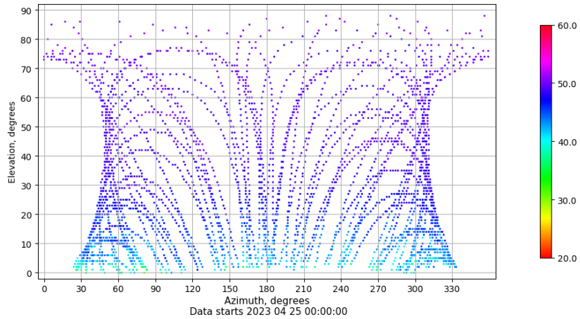
Azimuth-elevation plot for station RIO1. Signal to Noise S1C Data file RIO100ESP_R_2023115.xtr
