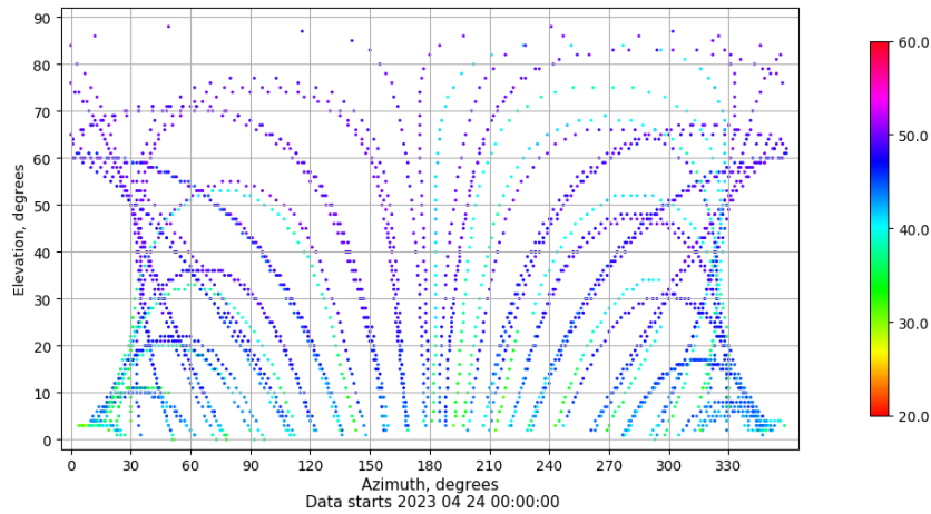
Azimuth-elevation plot for station RIO1. Signal to Noise S1C Data file RIO100ESP_R_2023114.xtr
