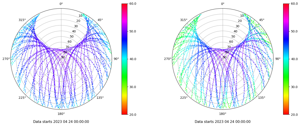
Skyplot for station RIO1. Signal to Noise S1C Data file RIO100ESP_R_2023114.xtr Skyplot for station RIO1. Signal to Noise S2W Data file RIO100ESP_R_2023114.xtr
