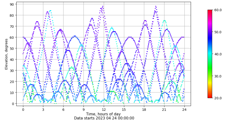
Time-elevation plot for station RIO1. Signal to Noise S1C Data file RIO100ESP_R_2023114.xtr
