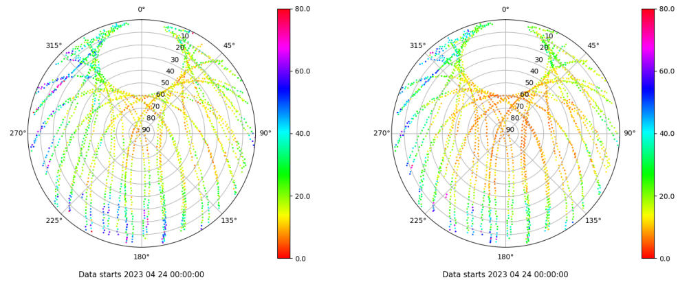
Skyplot for station RIO1. Parameter M1C Data file RIO100ESP_R_2023114.xtr Skyplot for station RIO1. Parameter M2P Data file RIO100ESP_R_2023114.xtr
