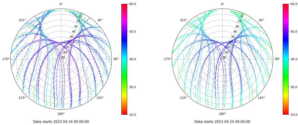
Skyplot for station RIO1. Signal to Noise S1C Data file RIO100ESP_R_2023114.xtr Skyplot for station RIO1. Signal to Noise S2P Data file RIO100ESP_R_2023114.xtr
