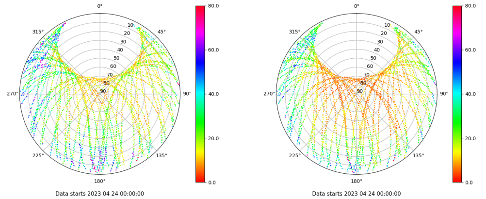
Skyplot for station RIO1. Parameter M1C Data file RIO100ESP_R_2023114.xtr Skyplot for station RIO1. Parameter M2W Data file RIO100ESP_R_2023114.xtr
