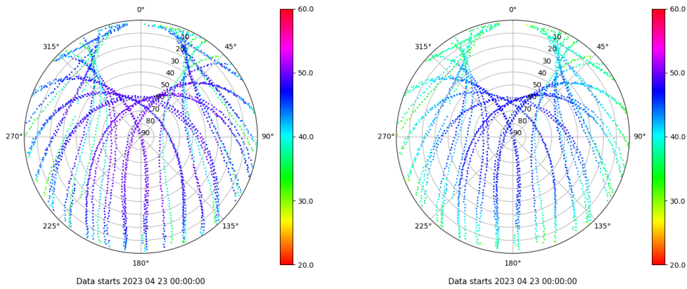
Skyplot for station RIO1. Signal to Noise S1C Data file RIO100ESP_R_2023113.xtr Skyplot for station RIO1. Signal to Noise S2P Data file RIO100ESP_R_2023113.xtr
