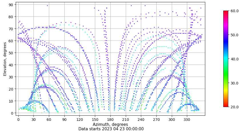
Azimuth-elevation plot for station RIO1. Signal to Noise S1C Data file RIO100ESP_R_2023113.xtr
