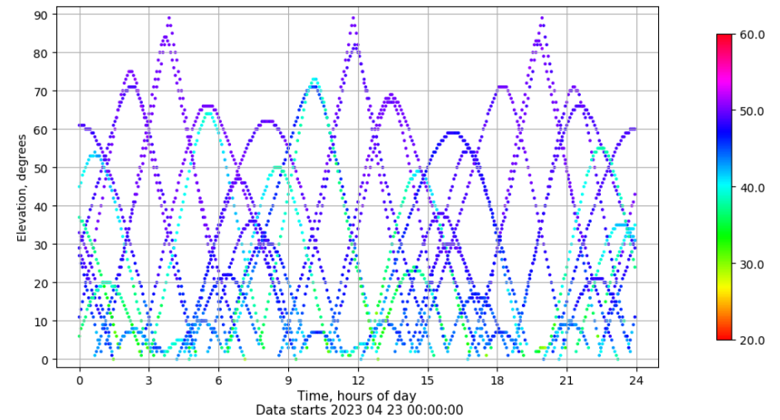
Time-elevation plot for station RIO1. Signal to Noise S1C Data file RIO100ESP_R_2023113.xtr
