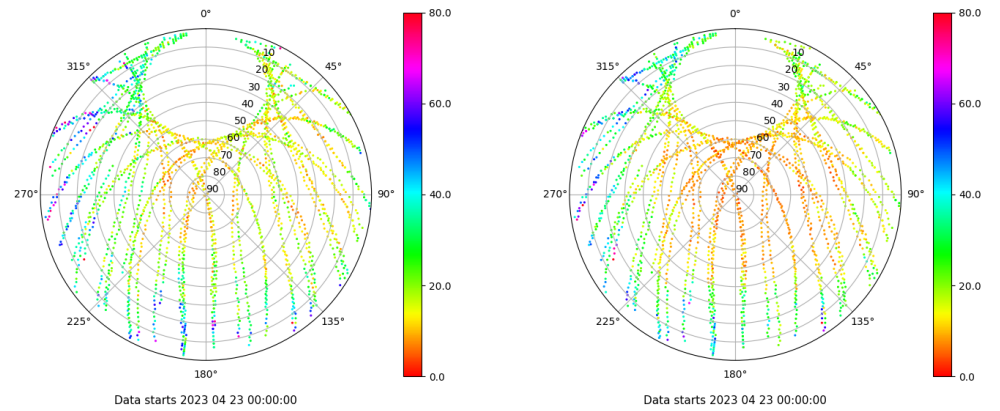
Skyplot for station RIO1. Parameter M1C Data file RIO100ESP_R_2023113.xtr Skyplot for station RIO1. Parameter M2P Data file RIO100ESP_R_2023113.xtr
