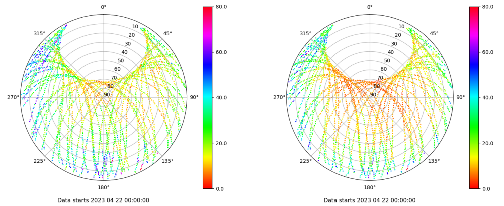
Skyplot for station RIO1. Parameter M1C Data file RIO100ESP_R_2023112.xtr Skyplot for station RIO1. Parameter M2W Data file RIO100ESP_R_2023112.xtr
