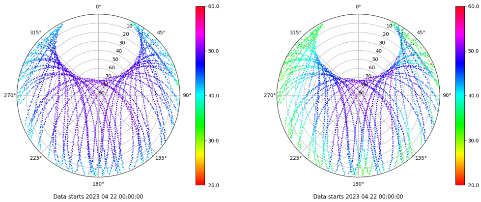
Skyplot for station RIO1. Signal to Noise S1C Data file RIO100ESP_R_2023112.xtr Skyplot for station RIO1. Signal to Noise S2W Data file RIO100ESP_R_2023112.xtr
