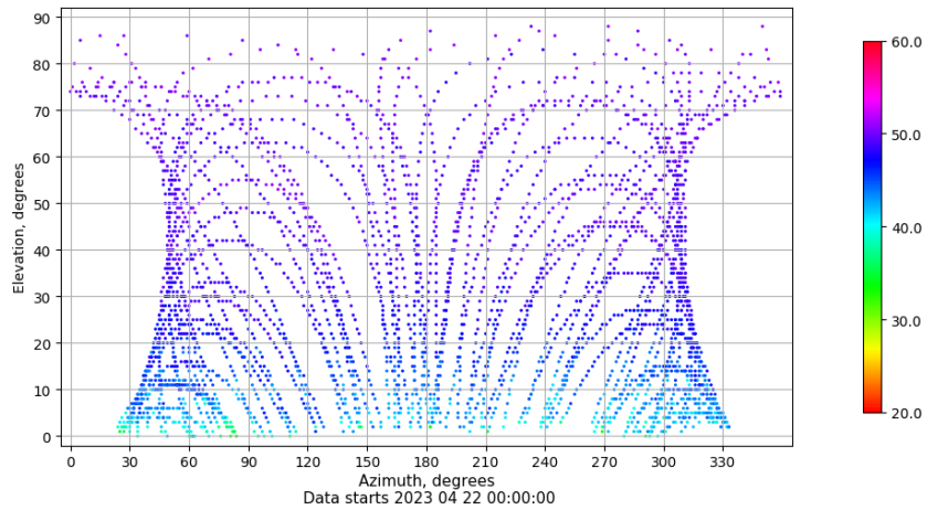
Azimuth-elevation plot for station RIO1. Signal to Noise S1C Data file RIO100ESP_R_2023112.xtr
