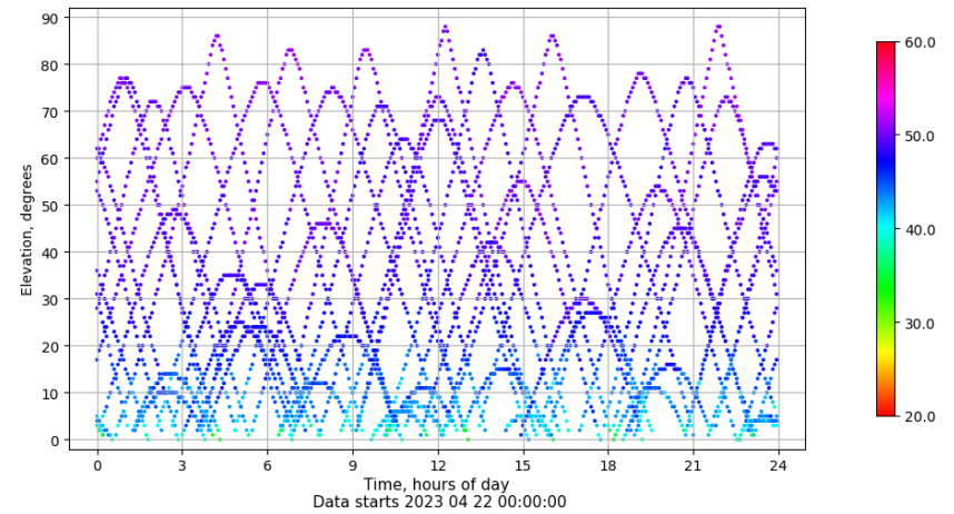
Time-elevation plot for station RIO1. Signal to Noise S1C Data file RIO100ESP_R_2023112.xtr
