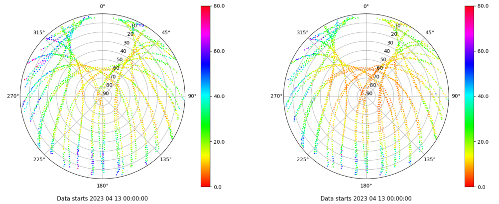
Skyplot for station RIO1. Parameter M1C Data file RIO100ESP_R_2023103.xtr Skyplot for station RIO1. Parameter M2P Data file RIO100ESP_R_2023103.xtr
