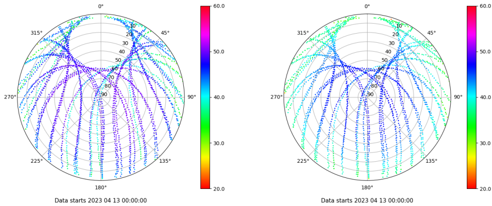
Skyplot for station RIO1. Signal to Noise S1C Data file RIO100ESP_R_2023103.xtr Skyplot for station RIO1. Signal to Noise S2P Data file RIO100ESP_R_2023103.xtr
