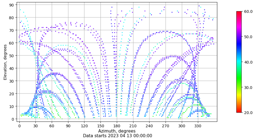
Azimuth-elevation plot for station RIO1. Signal to Noise S1C Data file RIO100ESP_R_2023103.xtr
