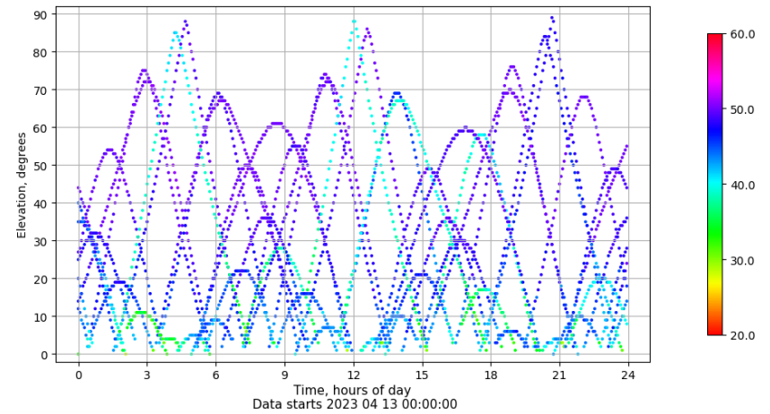
Time-elevation plot for station RIO1. Signal to Noise S1C Data file RIO100ESP_R_2023103.xtr
