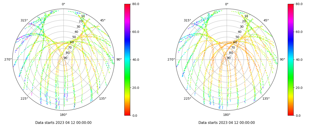
Skyplot for station RIO1. Parameter M1C Data file RIO100ESP_R_2023102.xtr Skyplot for station RIO1. Parameter M2P Data file RIO100ESP_R_2023102.xtr
