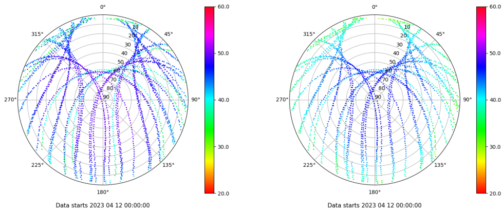
Skyplot for station RIO1. Signal to Noise S1C Data file RIO100ESP_R_2023102.xtr Skyplot for station RIO1. Signal to Noise S2P Data file RIO100ESP_R_2023102.xtr
