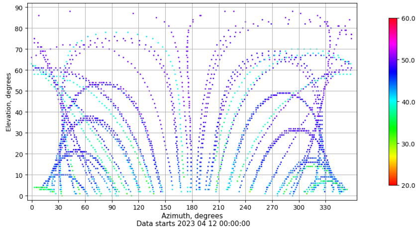
Azimuth-elevation plot for station RIO1. Signal to Noise S1C Data file RIO100ESP_R_2023102.xtr
