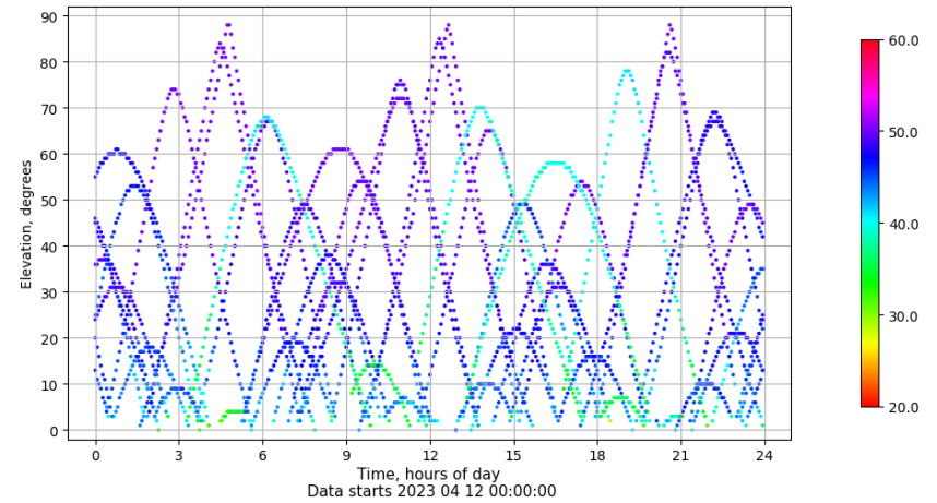
Time-elevation plot for station RIO1. Signal to Noise S1C Data file RIO100ESP_R_2023102.xtr
