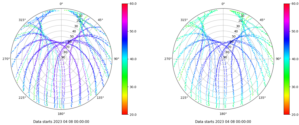
Skyplot for station RIO1. Signal to Noise S1C Data file RIO100ESP_R_2023098.xtr Skyplot for station RIO1. Signal to Noise S2P Data file RIO100ESP_R_2023098.xtr
