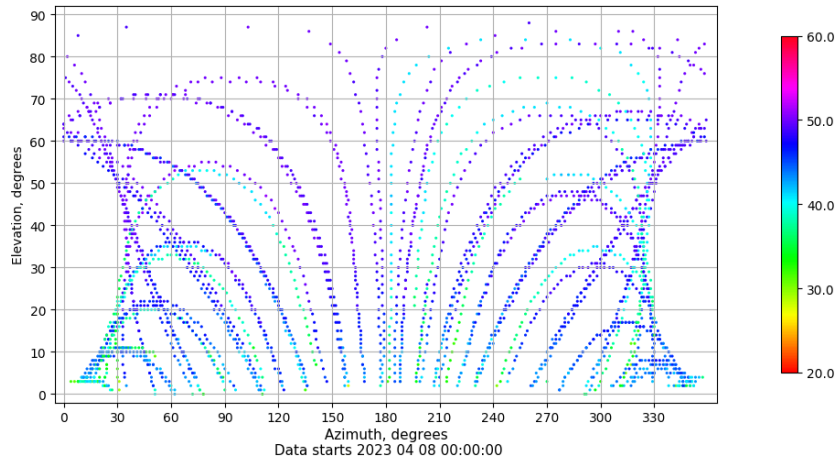
Azimuth-elevation plot for station RIO1. Signal to Noise S1C Data file RIO100ESP_R_2023098.xtr
