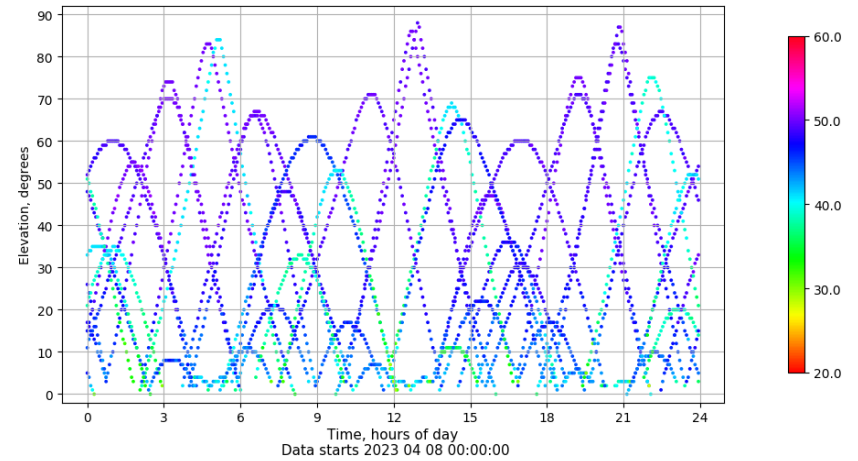
Time-elevation plot for station RIO1. Signal to Noise S1C Data file RIO100ESP_R_2023098.xtr
