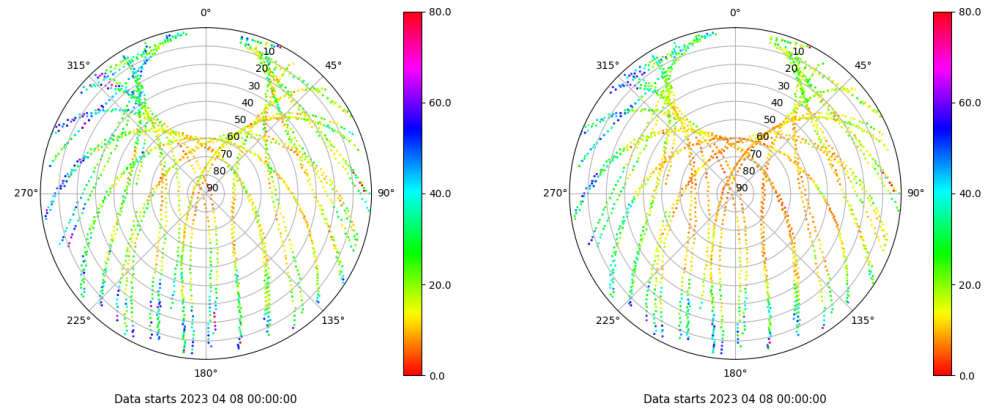
Skyplot for station RIO1. Parameter M1C Data file RIO100ESP_R_2023098.xtr Skyplot for station RIO1. Parameter M2P Data file RIO100ESP_R_2023098.xtr
