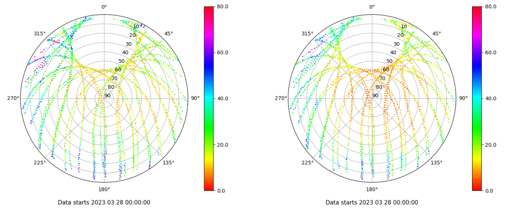
Skyplot for station RIO1. Parameter M1C Data file RIO100ESP_R_2023087.xtr Skyplot for station RIO1. Parameter M2P Data file RIO100ESP_R_2023087.xtr
