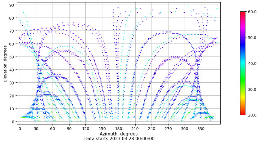
Azimuth-elevation plot for station RIO1. Signal to Noise S1C Data file RIO100ESP_R_2023087.xtr
