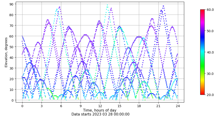
Time-elevation plot for station RIO1. Signal to Noise S1C Data file RIO100ESP_R_2023087.xtr
