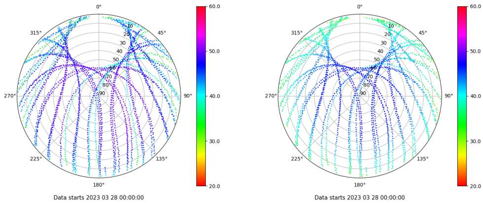
Skyplot for station RIO1. Signal to Noise S1C Data file RIO100ESP_R_2023087.xtr Skyplot for station RIO1. Signal to Noise S2P Data file RIO100ESP_R_2023087.xtr
