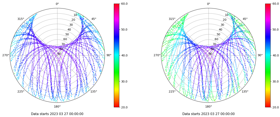
Skyplot for station RIO1. Signal to Noise S1C Data file RIO100ESP_R_2023086.xtr Skyplot for station RIO1. Signal to Noise S2W Data file RIO100ESP_R_2023086.xtr
