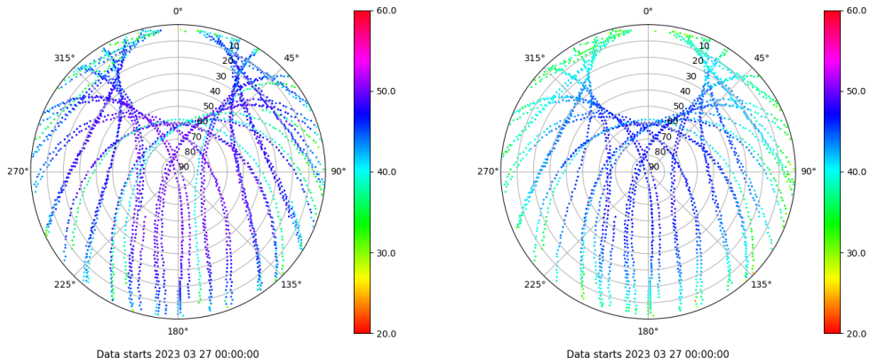
Skyplot for station RIO1. Signal to Noise S1C Data file RIO100ESP_R_2023086.xtr Skyplot for station RIO1. Signal to Noise S2P Data file RIO100ESP_R_2023086.xtr
