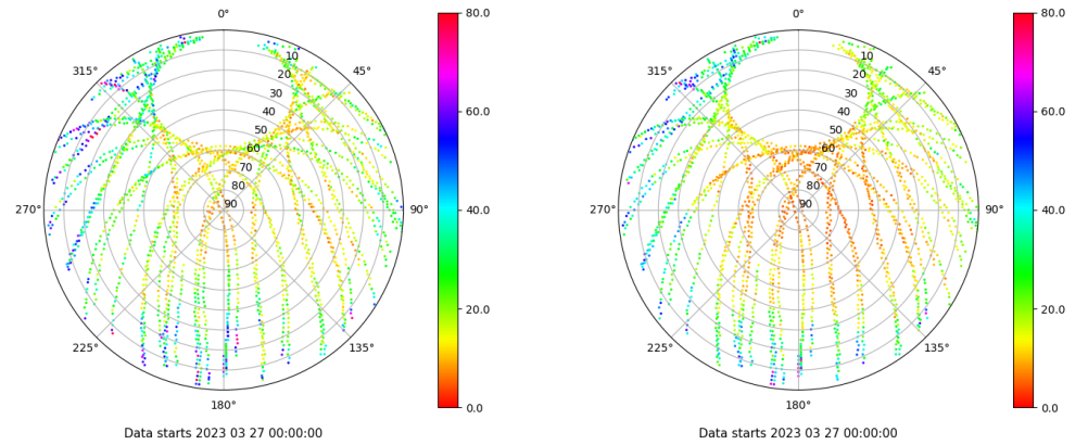
Skyplot for station RIO1. Parameter M1C Data file RIO100ESP_R_2023086.xtr Skyplot for station RIO1. Parameter M2P Data file RIO100ESP_R_2023086.xtr
