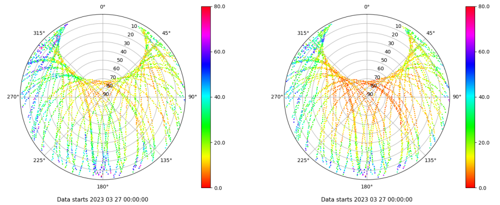
Skyplot for station RIO1. Parameter M1C Data file RIO100ESP_R_2023086.xtr Skyplot for station RIO1. Parameter M2W Data file RIO100ESP_R_2023086.xtr
