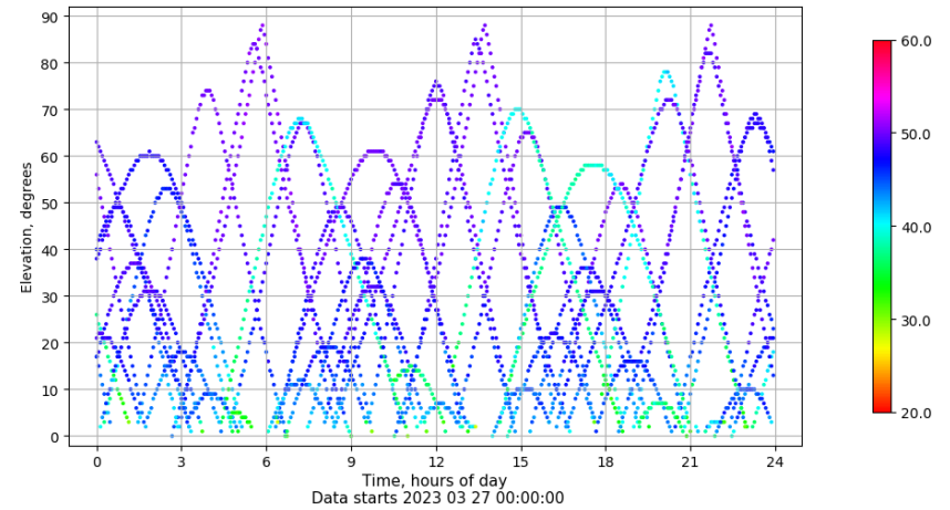
Time-elevation plot for station RIO1. Signal to Noise S1C Data file RIO100ESP_R_2023086.xtr
