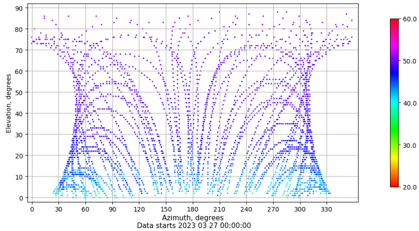
Azimuth-elevation plot for station RIO1. Signal to Noise S1C Data file RIO100ESP_R_2023086.xtr
