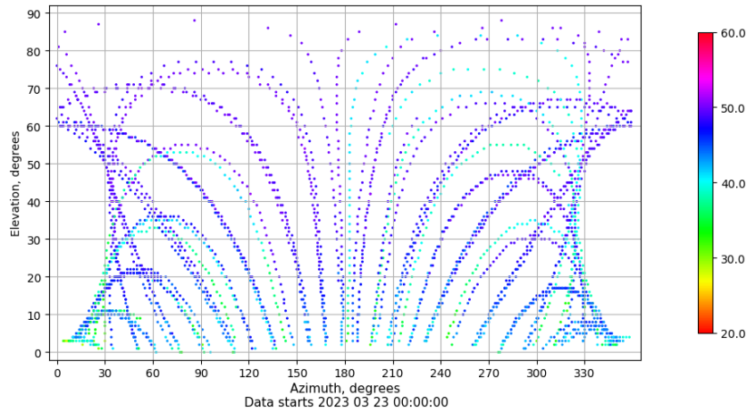
Azimuth-elevation plot for station RIO1. Signal to Noise S1C Data file RIO100ESP_R_2023082.xtr
