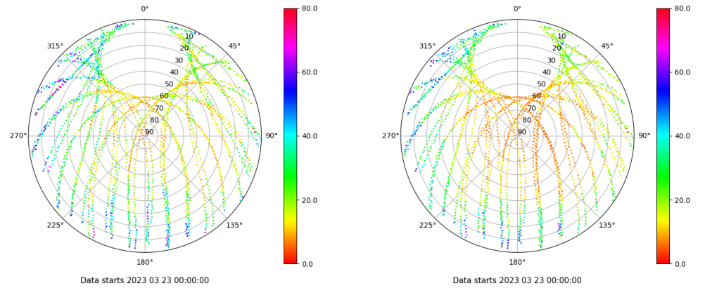
Skyplot for station RIO1. Parameter M1C Data file RIO100ESP_R_2023082.xtr Skyplot for station RIO1. Parameter M2P Data file RIO100ESP_R_2023082.xtr
