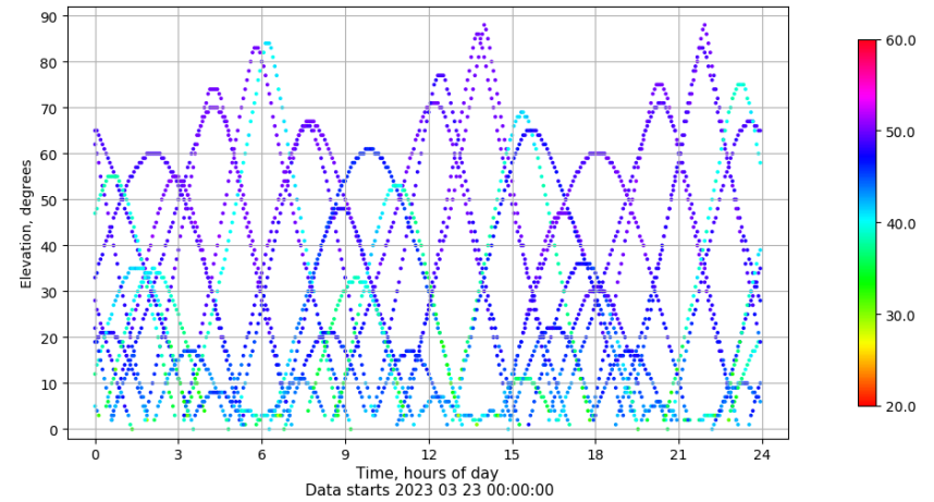
Time-elevation plot for station RIO1. Signal to Noise S1C Data file RIO100ESP_R_2023082.xtr
