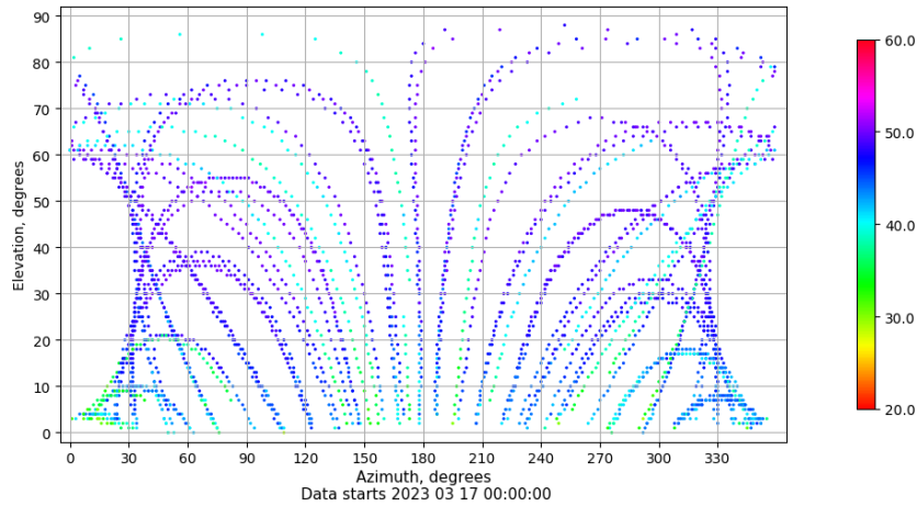
Azimuth-elevation plot for station RIO1. Signal to Noise S1C Data file RIO100ESP_R_2023076.xtr
