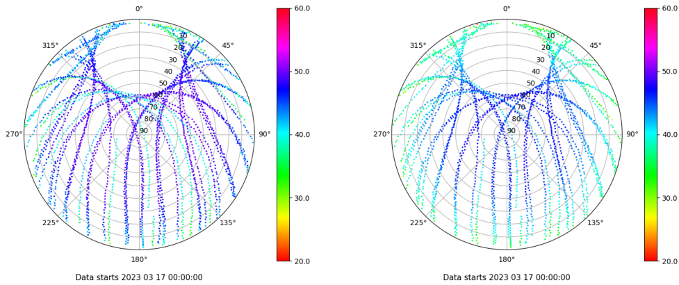
Skyplot for station RIO1. Signal to Noise S1C Data file RIO100ESP_R_2023076.xtr Skyplot for station RIO1. Signal to Noise S2P Data file RIO100ESP_R_2023076.xtr
