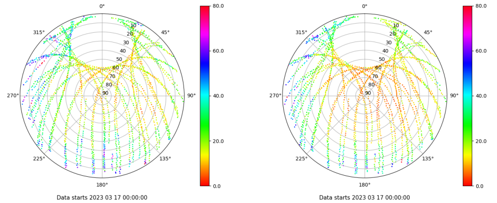
Skyplot for station RIO1. Parameter M1C Data file RIO100ESP_R_2023076.xtr Skyplot for station RIO1. Parameter M2P Data file RIO100ESP_R_2023076.xtr
