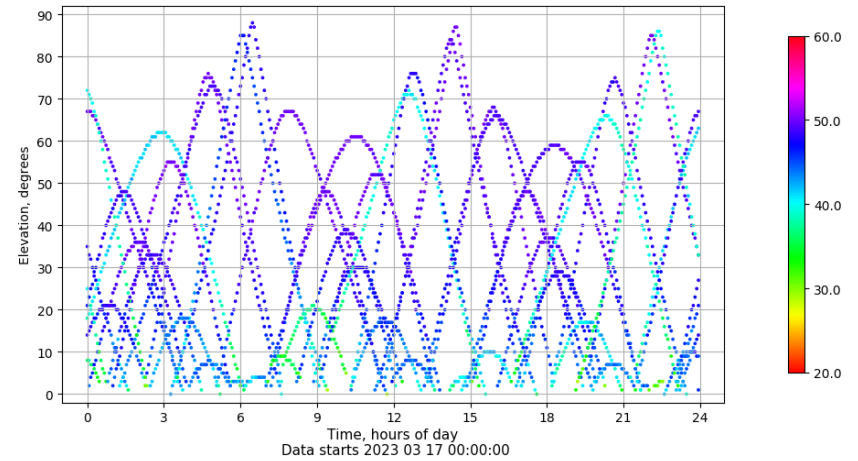
Time-elevation plot for station RIO1. Signal to Noise S1C Data file RIO100ESP_R_2023076.xtr
