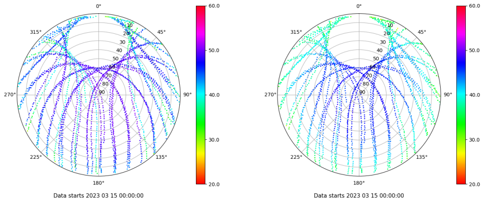
Skyplot for station RIO1. Signal to Noise S1C Data file RIO100ESP_R_2023074.xtr Skyplot for station RIO1. Signal to Noise S2P Data file RIO100ESP_R_2023074.xtr
