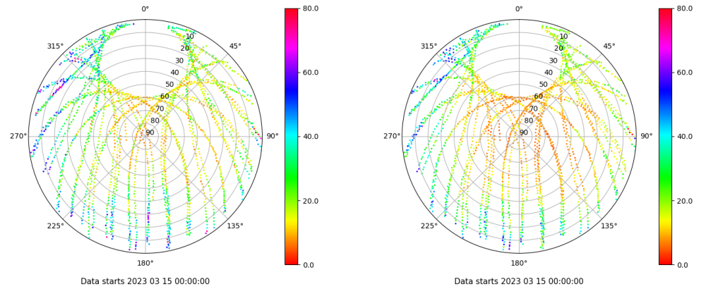
Skyplot for station RIO1. Parameter M1C Data file RIO100ESP_R_2023074.xtr Skyplot for station RIO1. Parameter M2P Data file RIO100ESP_R_2023074.xtr
