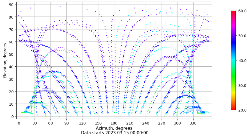
Azimuth-elevation plot for station RIO1. Signal to Noise S1C Data file RIO100ESP_R_2023074.xtr
