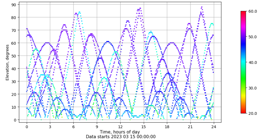
Time-elevation plot for station RIO1. Signal to Noise S1C Data file RIO100ESP_R_2023074.xtr
