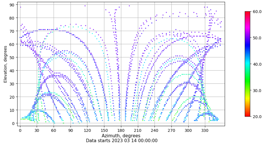
Azimuth-elevation plot for station RIO1. Signal to Noise S1C Data file RIO100ESP_R_2023073.xtr
