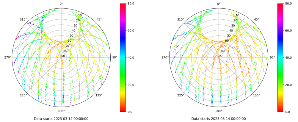
Skyplot for station RIO1. Parameter M1C Data file RIO100ESP_R_2023073.xtr Skyplot for station RIO1. Parameter M2P Data file RIO100ESP_R_2023073.xtr
