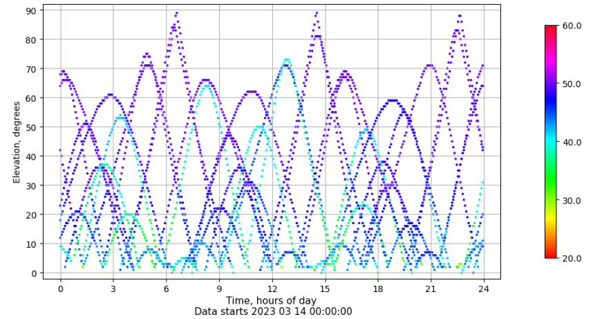
Time-elevation plot for station RIO1. Signal to Noise S1C Data file RIO100ESP_R_2023073.xtr
