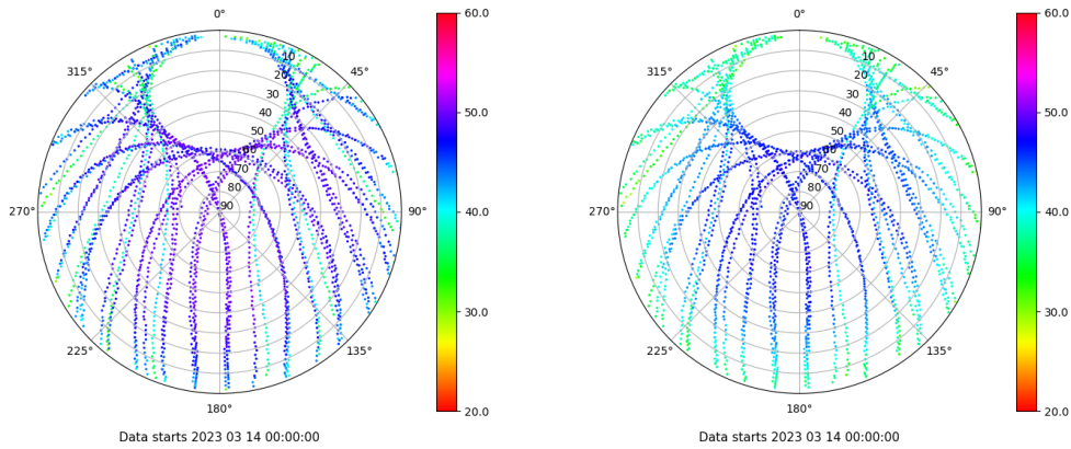
Skyplot for station RIO1. Signal to Noise S1C Data file RIO100ESP_R_2023073.xtr Skyplot for station RIO1. Signal to Noise S2P Data file RIO100ESP_R_2023073.xtr
