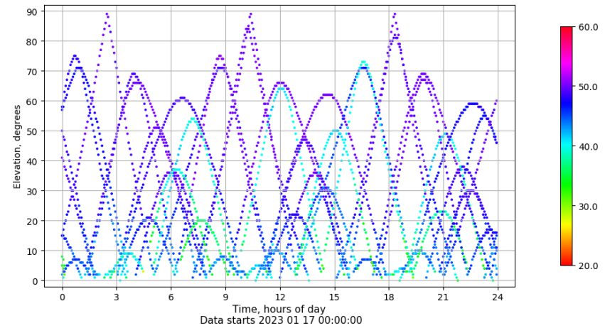
Time-elevation plot for station RIO1. Signal to Noise S1C Data file RIO100ESP_R_2023017.xtr
