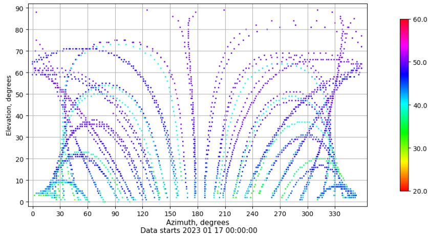
Azimuth-elevation plot for station RIO1. Signal to Noise S1C Data file RIO100ESP_R_2023017.xtr
