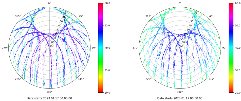
Skyplot for station RIO1. Signal to Noise S1C Data file RIO100ESP_R_2023017.xtr Skyplot for station RIO1. Signal to Noise S2P Data file RIO100ESP_R_2023017.xtr
