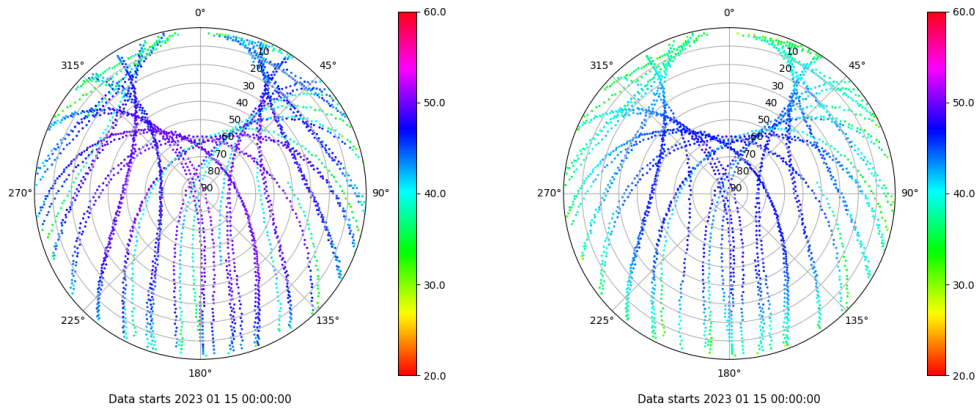
Skyplot for station RIO1. Signal to Noise S1C Data file RIO100ESP_R_2023015.xtr Skyplot for station RIO1. Signal to Noise S2P Data file RIO100ESP_R_2023015.xtr
