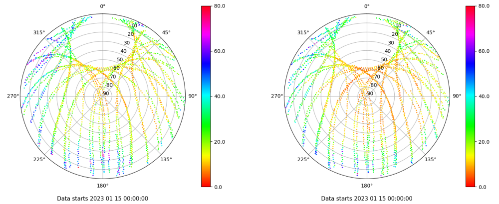
Skyplot for station RIO1. Parameter M1C Data file RIO100ESP_R_2023015.xtr Skyplot for station RIO1. Parameter M2P Data file RIO100ESP_R_2023015.xtr
