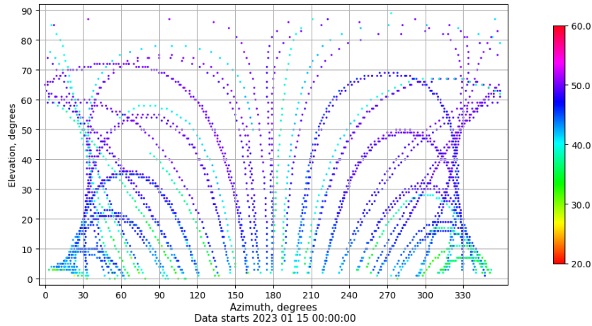
Azimuth-elevation plot for station RIO1. Signal to Noise S1C Data file RIO100ESP_R_2023015.xtr
