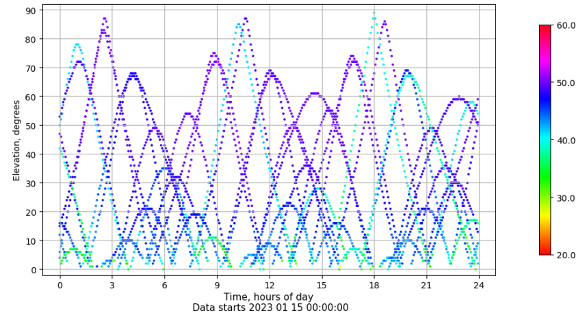
Time-elevation plot for station RIO1. Signal to Noise S1C Data file RIO100ESP_R_2023015.xtr
