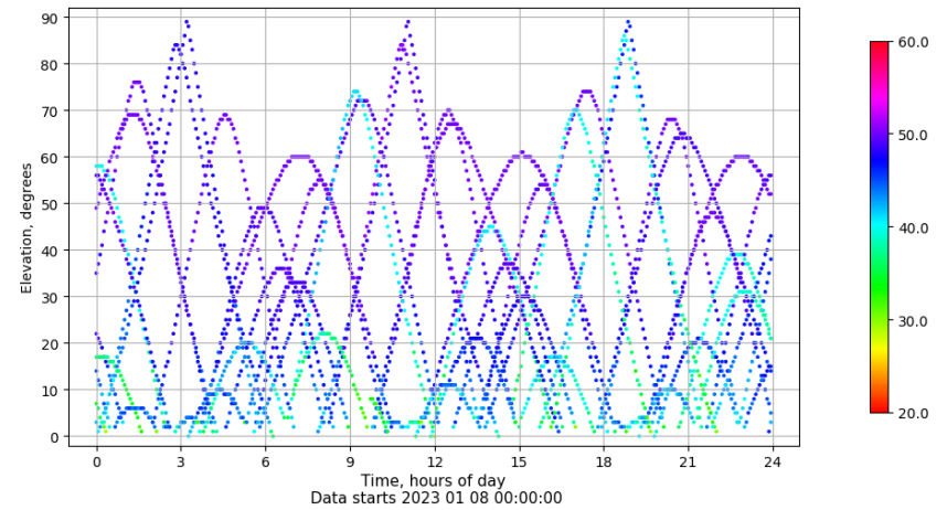
Time-elevation plot for station RIO1. Signal to Noise S1C Data file RIO100ESP_R_2023008.xtr
