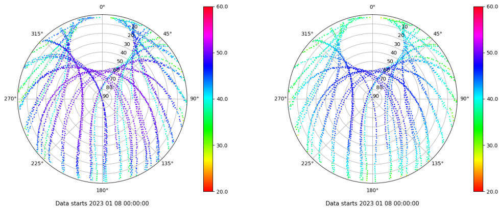
Skyplot for station RIO1. Signal to Noise S1C Data file RIO100ESP_R_2023008.xtr Skyplot for station RIO1. Signal to Noise S2P Data file RIO100ESP_R_2023008.xtr
