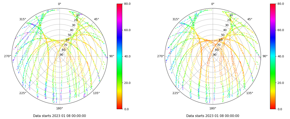
Skyplot for station RIO1. Parameter M1C Data file RIO100ESP_R_2023008.xtr Skyplot for station RIO1. Parameter M2P Data file RIO100ESP_R_2023008.xtr
