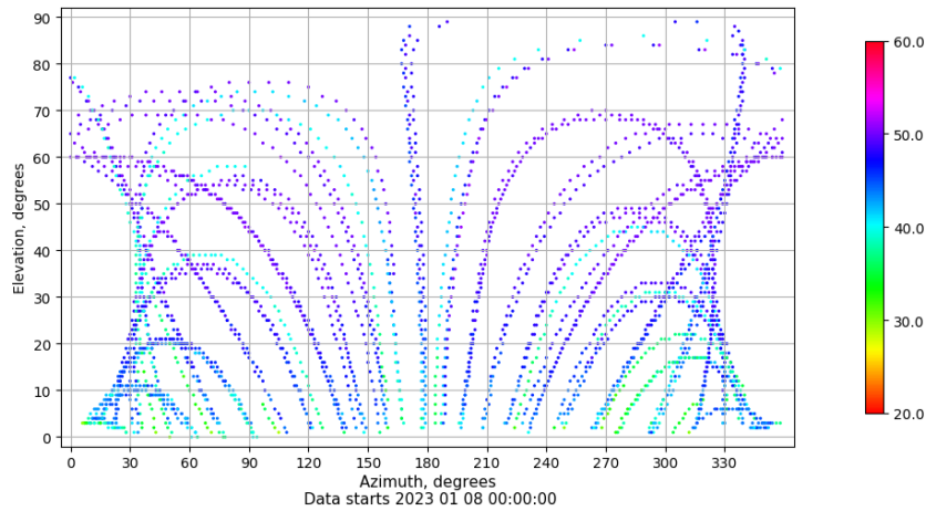
Azimuth-elevation plot for station RIO1. Signal to Noise S1C Data file RIO100ESP_R_2023008.xtr
