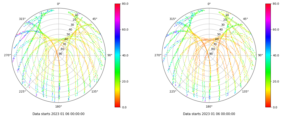
Skyplot for station RIO1. Parameter M1C Data file RIO100ESP_R_2023006.xtr Skyplot for station RIO1. Parameter M2P Data file RIO100ESP_R_2023006.xtr
