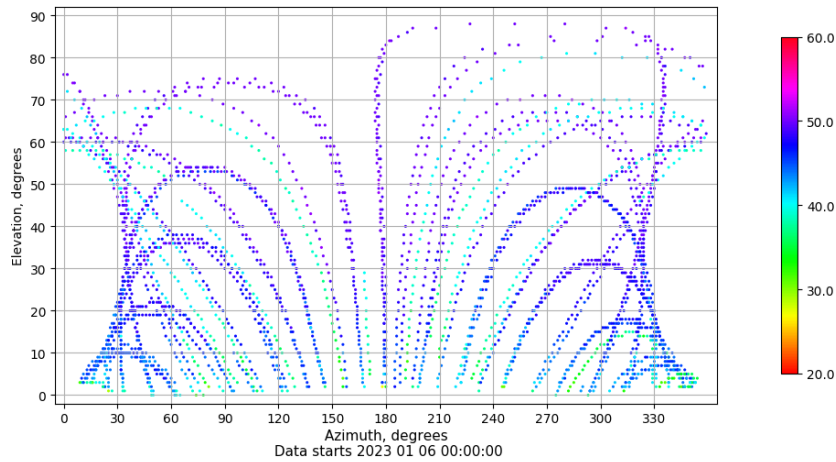
Azimuth-elevation plot for station RIO1. Signal to Noise S1C Data file RIO100ESP_R_2023006.xtr
