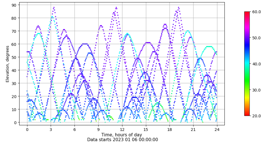
Time-elevation plot for station RIO1. Signal to Noise S1C Data file RIO100ESP_R_2023006.xtr
