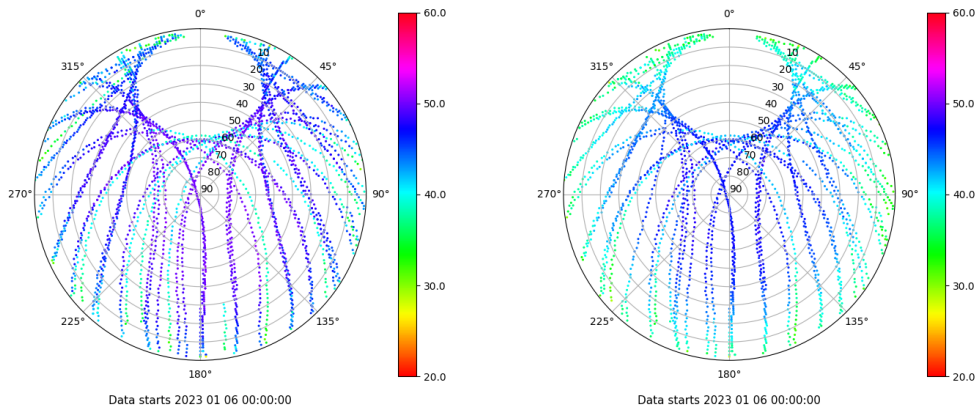
Skyplot for station RIO1. Signal to Noise S1C Data file RIO100ESP_R_2023006.xtr Skyplot for station RIO1. Signal to Noise S2P Data file RIO100ESP_R_2023006.xtr
