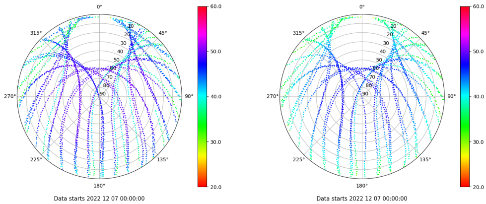
Skyplot for station RIO1. Signal to Noise S1C Data file RIO100ESP_R_2022341.xtr Skyplot for station RIO1. Signal to Noise S2P Data file RIO100ESP_R_2022341.xtr
