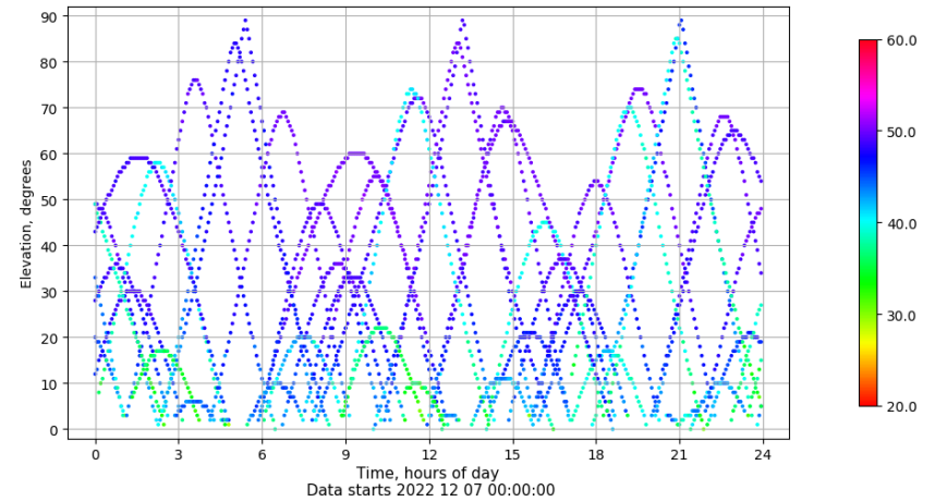
Time-elevation plot for station RIO1. Signal to Noise S1C Data file RIO100ESP_R_2022341.xtr
