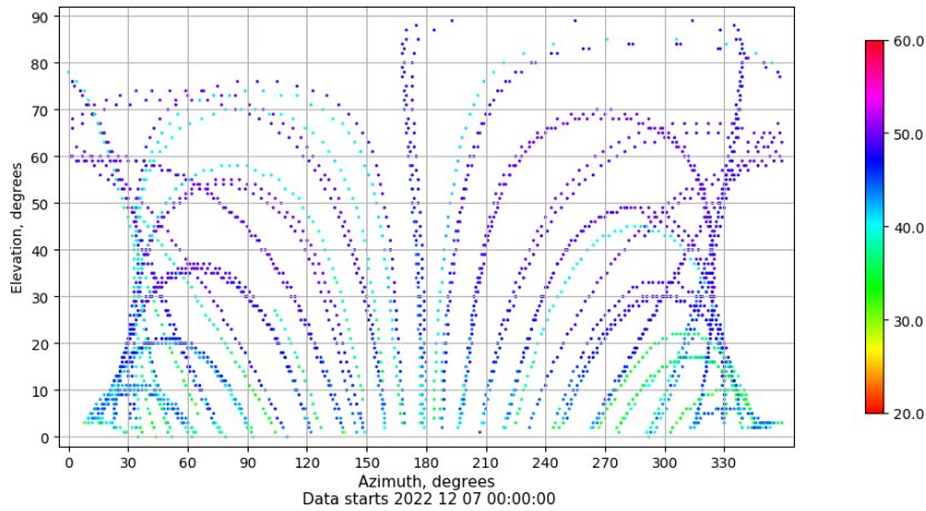
Azimuth-elevation plot for station RIO1. Signal to Noise S1C Data file RIO100ESP_R_2022341.xtr
