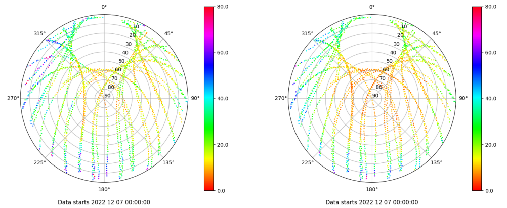
Skyplot for station RIO1. Parameter M1C Data file RIO100ESP_R_2022341.xtr Skyplot for station RIO1. Parameter M2P Data file RIO100ESP_R_2022341.xtr
