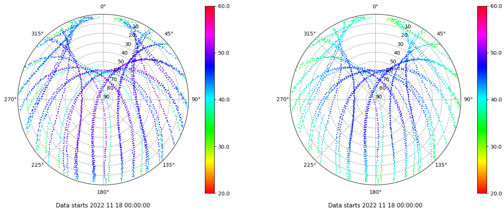
Skyplot for station RIO1. Signal to Noise S1C Data file RIO100ESP_R_2022322.xtr Skyplot for station RIO1. Signal to Noise S2P Data file RIO100ESP_R_2022322.xtr
