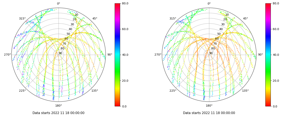
Skyplot for station RIO1. Parameter M1C Data file RIO100ESP_R_2022322.xtr Skyplot for station RIO1. Parameter M2P Data file RIO100ESP_R_2022322.xtr
