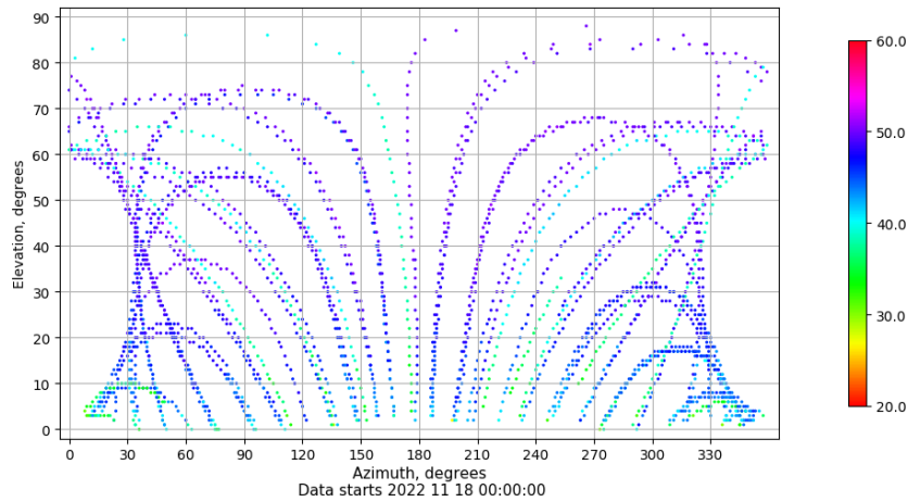
Azimuth-elevation plot for station RIO1. Signal to Noise S1C Data file RIO100ESP_R_2022322.xtr
