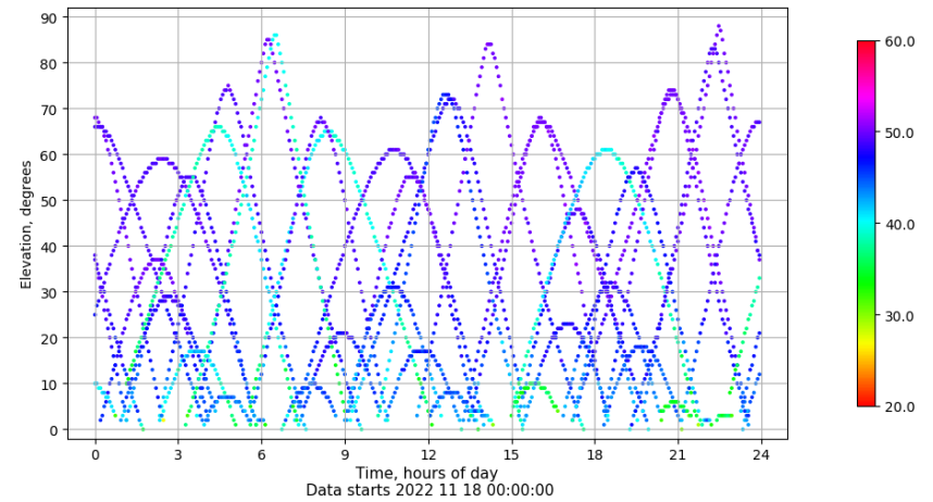
Time-elevation plot for station RIO1. Signal to Noise S1C Data file RIO100ESP_R_2022322.xtr
