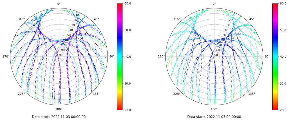
Skyplot for station RIO1. Signal to Noise S1C Data file RIO100ESP_R_2022307.xtr Skyplot for station RIO1. Signal to Noise S2P Data file RIO100ESP_R_2022307.xtr
