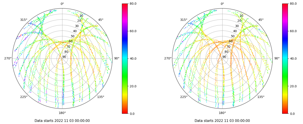
Skyplot for station RIO1. Parameter M1C Data file RIO100ESP_R_2022307.xtr Skyplot for station RIO1. Parameter M2P Data file RIO100ESP_R_2022307.xtr
