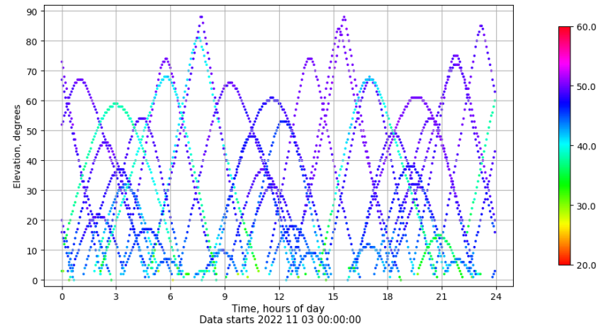
Time-elevation plot for station RIO1. Signal to Noise S1C Data file RIO100ESP_R_2022307.xtr
