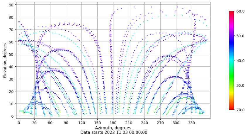
Azimuth-elevation plot for station RIO1. Signal to Noise S1C Data file RIO100ESP_R_2022307.xtr
