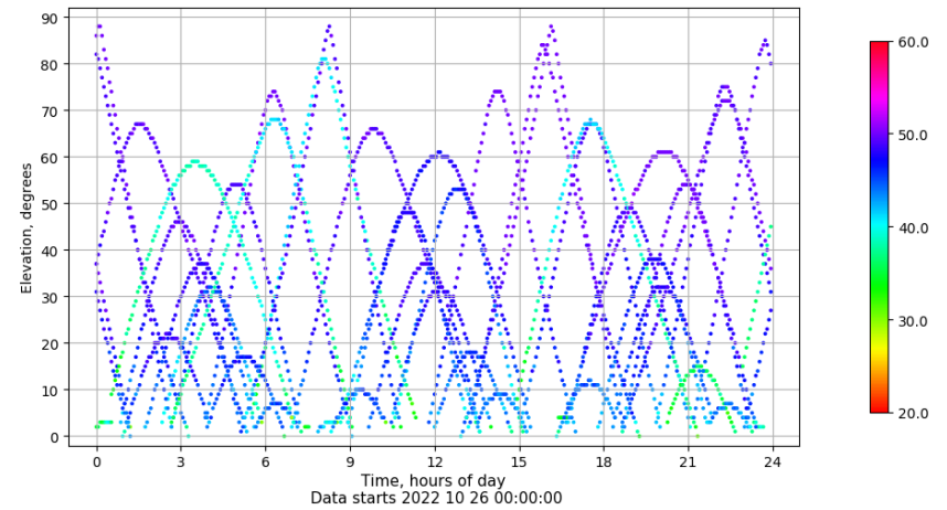
Time-elevation plot for station RIO1. Signal to Noise S1C Data file RIO100ESP_R_2022299.xtr
