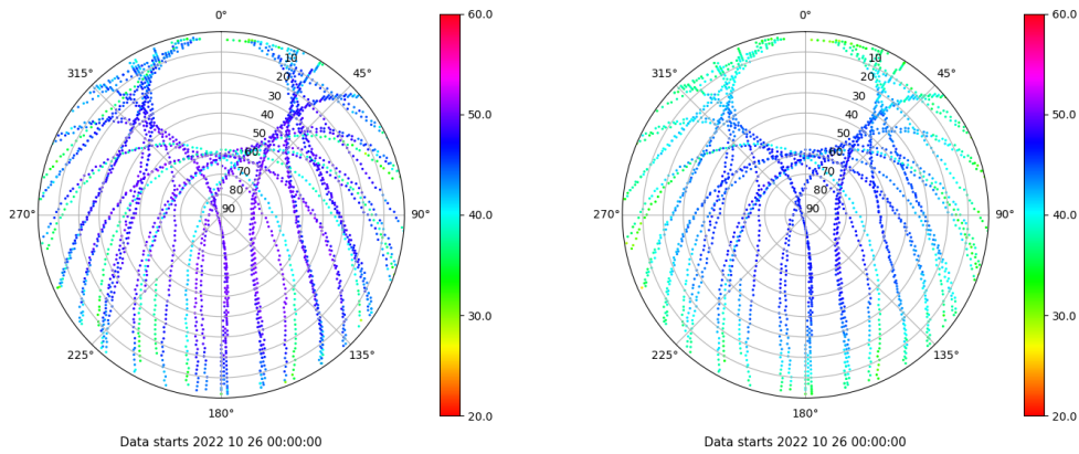
Skyplot for station RIO1. Signal to Noise S1C Data file RIO100ESP_R_2022299.xtr Skyplot for station RIO1. Signal to Noise S2P Data file RIO100ESP_R_2022299.xtr
