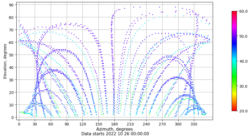
Azimuth-elevation plot for station RIO1. Signal to Noise S1C Data file RIO100ESP_R_2022299.xtr
