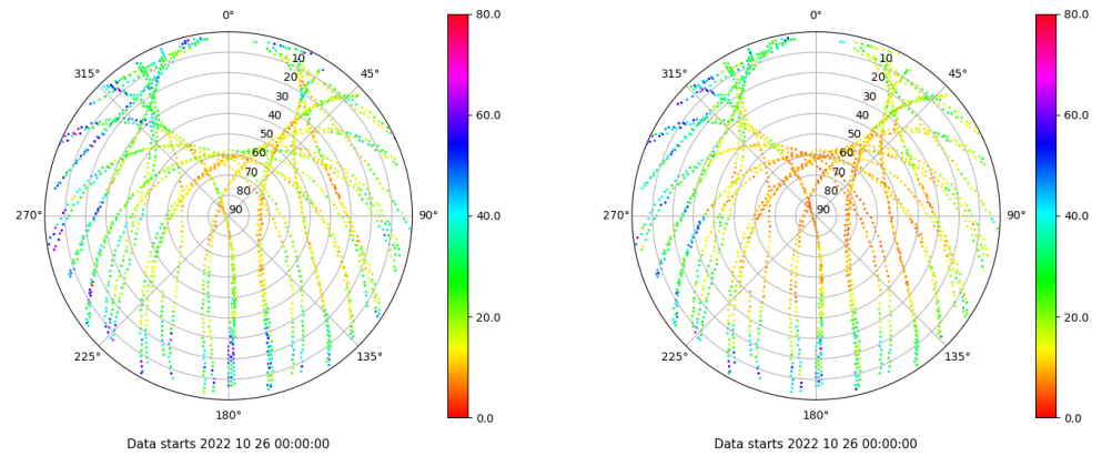
Skyplot for station RIO1. Parameter M1C Data file RIO100ESP_R_2022299.xtr Skyplot for station RIO1. Parameter M2P Data file RIO100ESP_R_2022299.xtr
