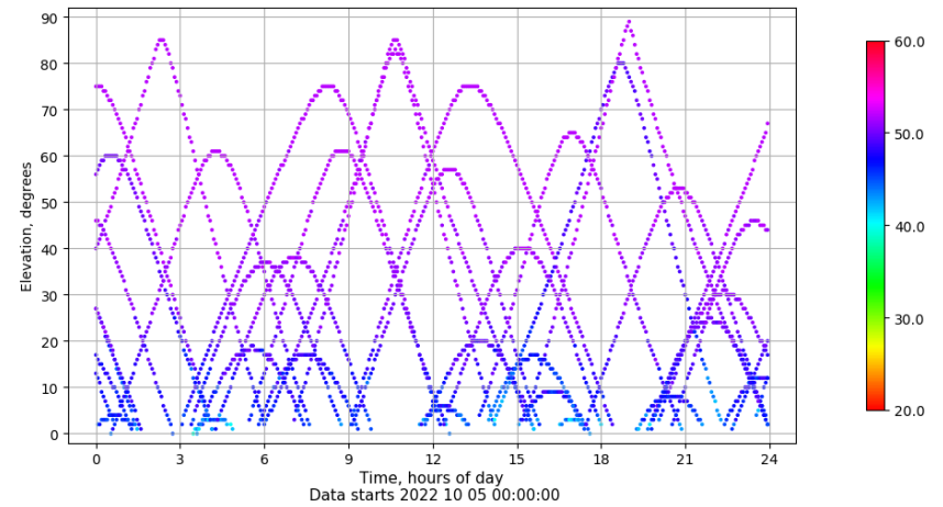
Time-elevation plot for station RIO1. Signal to Noise S1C Data file RIO100ESP_R_2022278.xtr
