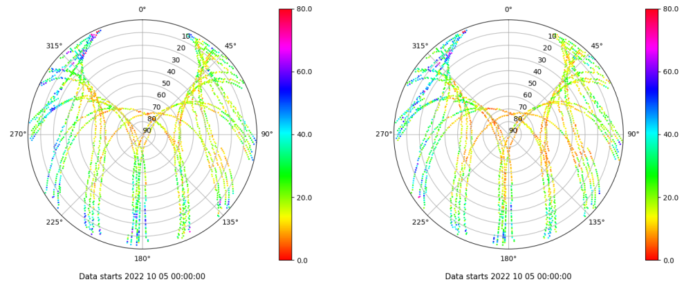
Skyplot for station RIO1. Parameter M1C Data file RIO100ESP_R_2022278.xtr Skyplot for station RIO1. Parameter M5Q Data file RIO100ESP_R_2022278.xtr
