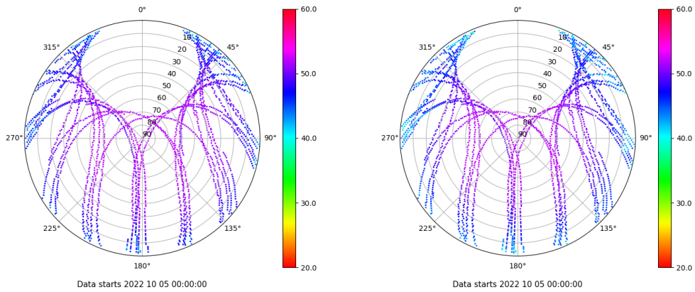
Skyplot for station RIO1. Signal to Noise S1C Data file RIO100ESP_R_2022278.xtr Skyplot for station RIO1. Signal to Noise S5Q Data file RIO100ESP_R_2022278.xtr
