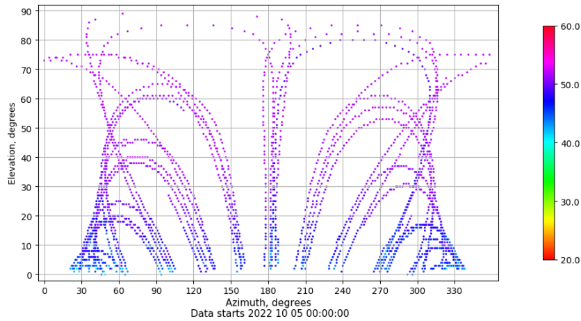
Azimuth-elevation plot for station RIO1. Signal to Noise S1C Data file RIO100ESP_R_2022278.xtr
