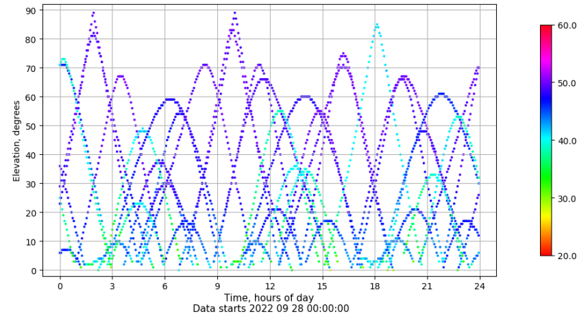
Time-elevation plot for station RIO1. Signal to Noise S1C Data file RIO100ESP_R_2022271.xtr
