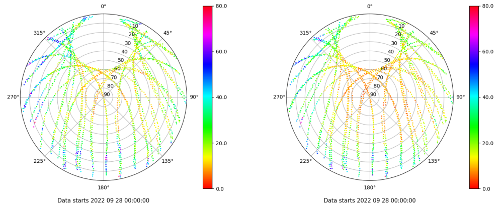
Skyplot for station RIO1. Parameter M1C Data file RIO100ESP_R_2022271.xtr Skyplot for station RIO1. Parameter M2P Data file RIO100ESP_R_2022271.xtr
