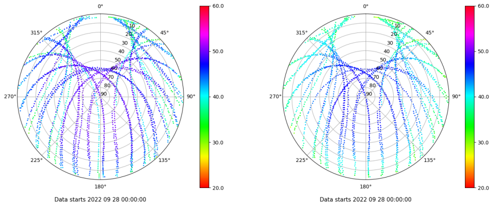
Skyplot for station RIO1. Signal to Noise S1C Data file RIO100ESP_R_2022271.xtr Skyplot for station RIO1. Signal to Noise S2P Data file RIO100ESP_R_2022271.xtr
