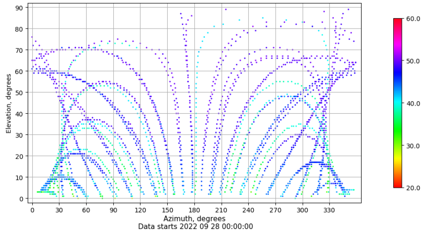
Azimuth-elevation plot for station RIO1. Signal to Noise S1C Data file RIO100ESP_R_2022271.xtr
