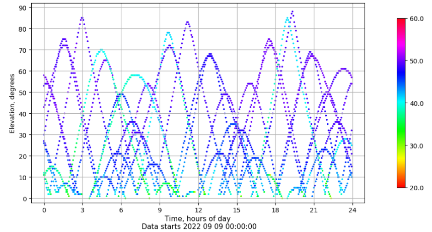
Time-elevation plot for station RIO1. Signal to Noise S1C Data file RIO100ESP_R_2022252.xtr
