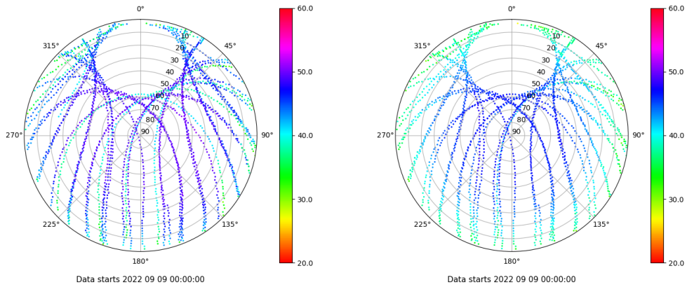
Skyplot for station RIO1. Signal to Noise S1C Data file RIO100ESP_R_2022252.xtr Skyplot for station RIO1. Signal to Noise S2P Data file RIO100ESP_R_2022252.xtr
