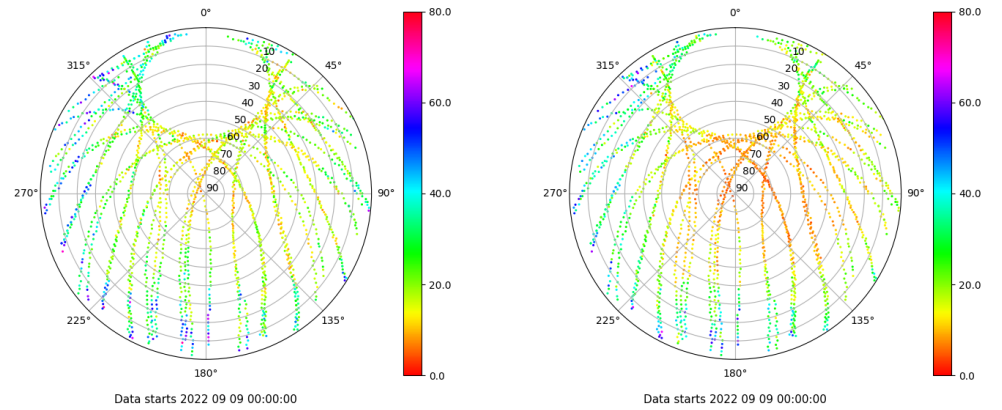
Skyplot for station RIO1. Parameter M1C Data file RIO100ESP_R_2022252.xtr Skyplot for station RIO1. Parameter M2P Data file RIO100ESP_R_2022252.xtr
