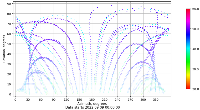
Azimuth-elevation plot for station RIO1. Signal to Noise S1C Data file RIO100ESP_R_2022252.xtr
