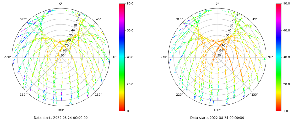
Skyplot for station RIO1. Parameter M1C Data file RIO100ESP_R_2022236.xtr Skyplot for station RIO1. Parameter M2P Data file RIO100ESP_R_2022236.xtr
