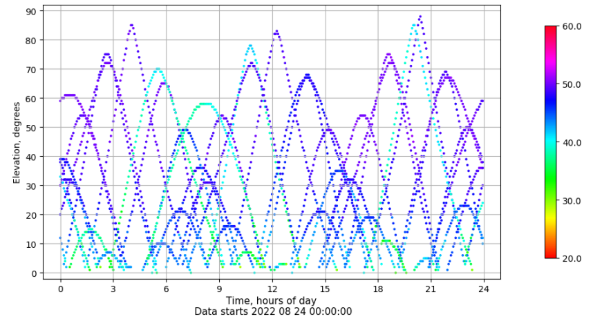
Time-elevation plot for station RIO1. Signal to Noise S1C Data file RIO100ESP_R_2022236.xtr
