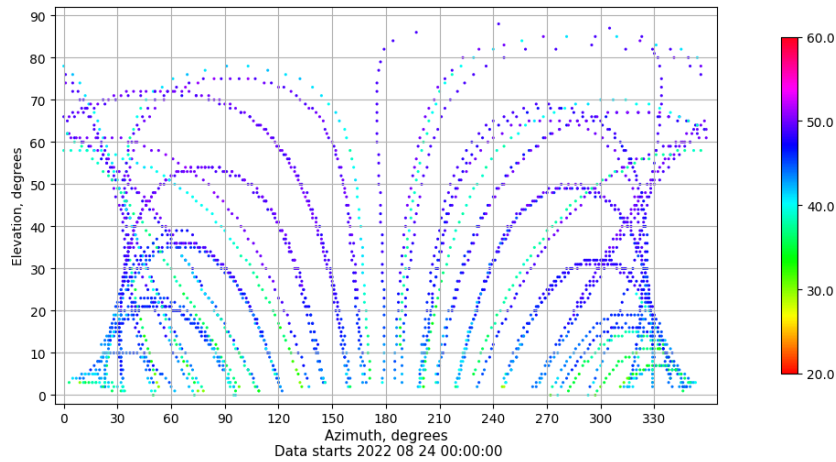
Azimuth-elevation plot for station RIO1. Signal to Noise S1C Data file RIO100ESP_R_2022236.xtr
