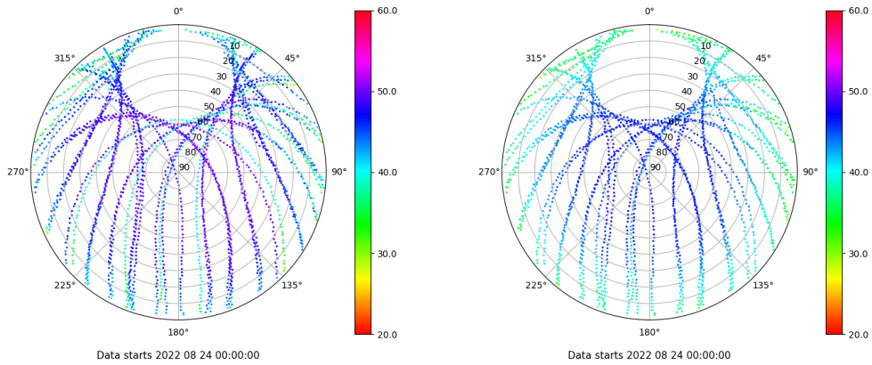
Skyplot for station RIO1. Signal to Noise S1C Data file RIO100ESP_R_2022236.xtr Skyplot for station RIO1. Signal to Noise S2P Data file RIO100ESP_R_2022236.xtr
