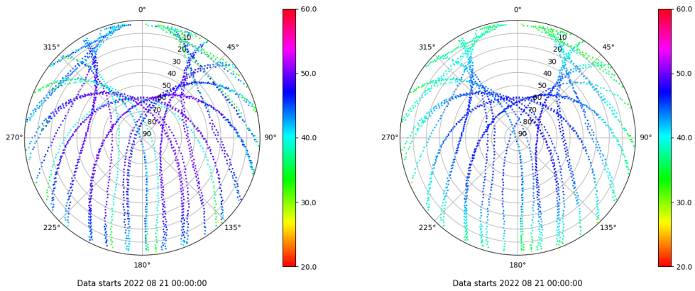
Skyplot for station RIO1. Signal to Noise S1C Data file RIO100ESP_R_2022233.xtr Skyplot for station RIO1. Signal to Noise S2P Data file RIO100ESP_R_2022233.xtr
