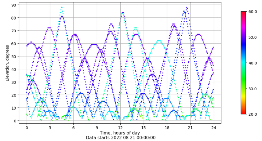
Time-elevation plot for station RIO1. Signal to Noise S1C Data file RIO100ESP_R_2022233.xtr
