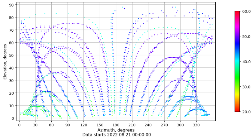
Azimuth-elevation plot for station RIO1. Signal to Noise S1C Data file RIO100ESP_R_2022233.xtr
