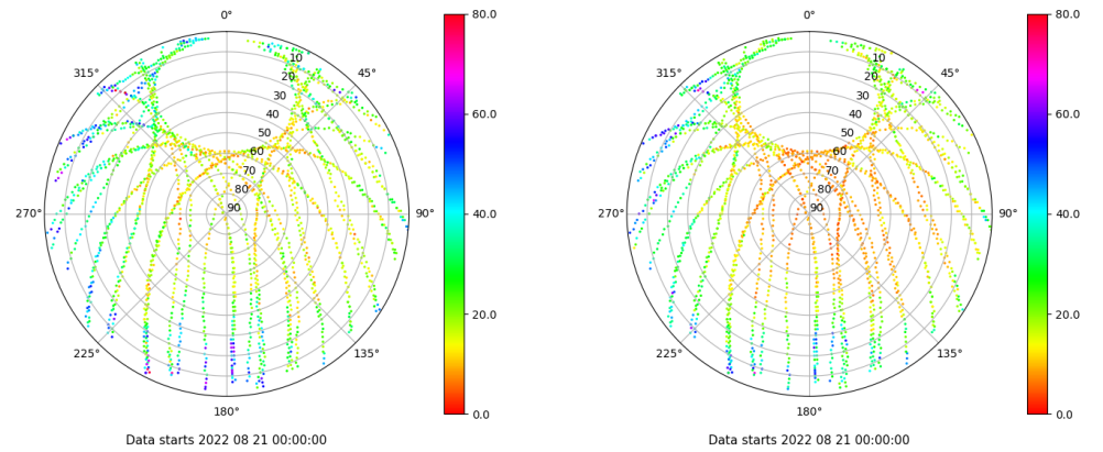
Skyplot for station RIO1. Parameter M1C Data file RIO100ESP_R_2022233.xtr Skyplot for station RIO1. Parameter M2P Data file RIO100ESP_R_2022233.xtr
