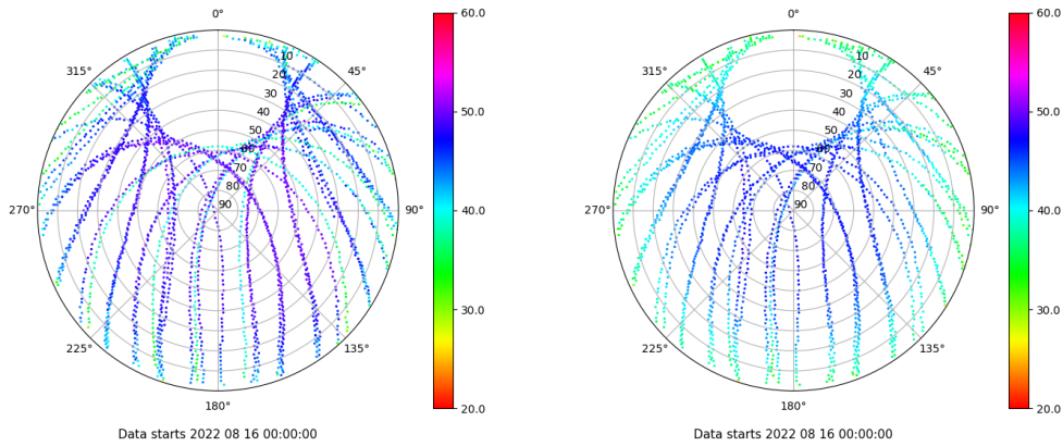
Skyplot for station RIO1. Signal to Noise S1C Data file RIO100ESP_R_2022228.xtr Skyplot for station RIO1. Signal to Noise S2P Data file RIO100ESP_R_2022228.xtr
