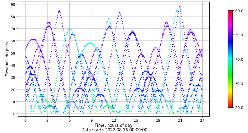
Time-elevation plot for station RIO1. Signal to Noise S1C Data file RIO100ESP_R_2022228.xtr
