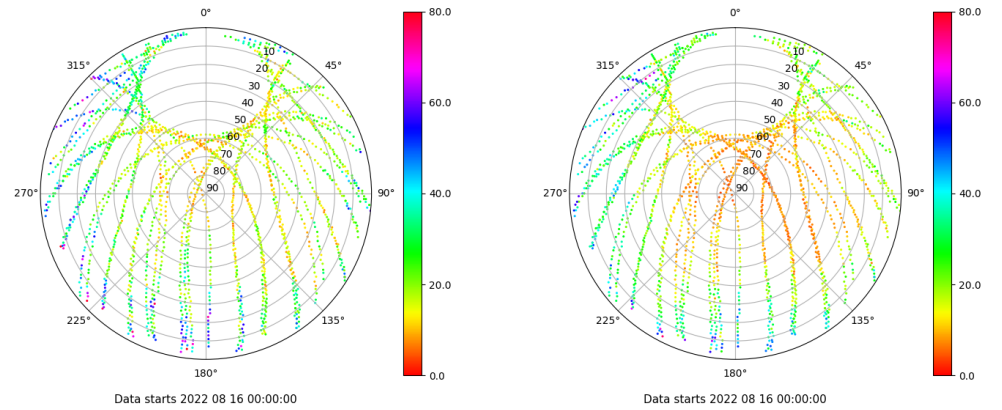
Skyplot for station RIO1. Parameter M1C Data file RIO100ESP_R_2022228.xtr Skyplot for station RIO1. Parameter M2P Data file RIO100ESP_R_2022228.xtr
