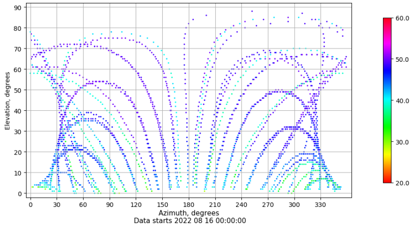
Azimuth-elevation plot for station RIO1. Signal to Noise S1C Data file RIO100ESP_R_2022228.xtr
