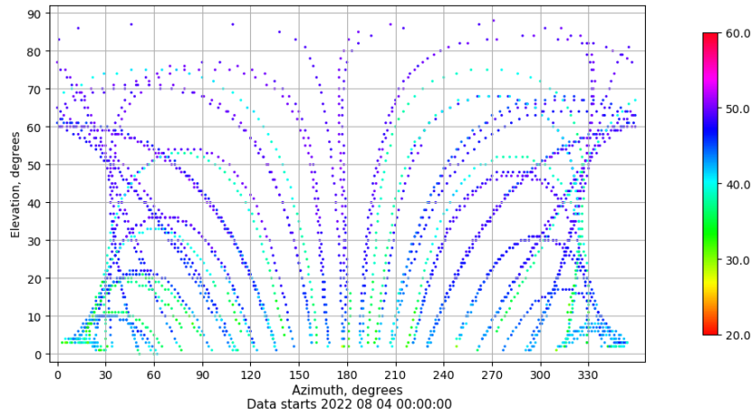
Azimuth-elevation plot for station RIO1. Signal to Noise S1C Data file RIO100ESP_R_2022216.xtr
