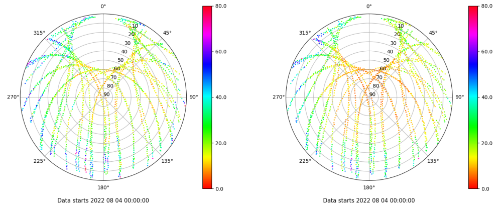
Skyplot for station RIO1. Parameter M1C Data file RIO100ESP_R_2022216.xtr Skyplot for station RIO1. Parameter M2P Data file RIO100ESP_R_2022216.xtr
