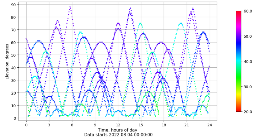
Time-elevation plot for station RIO1. Signal to Noise S1C Data file RIO100ESP_R_2022216.xtr
