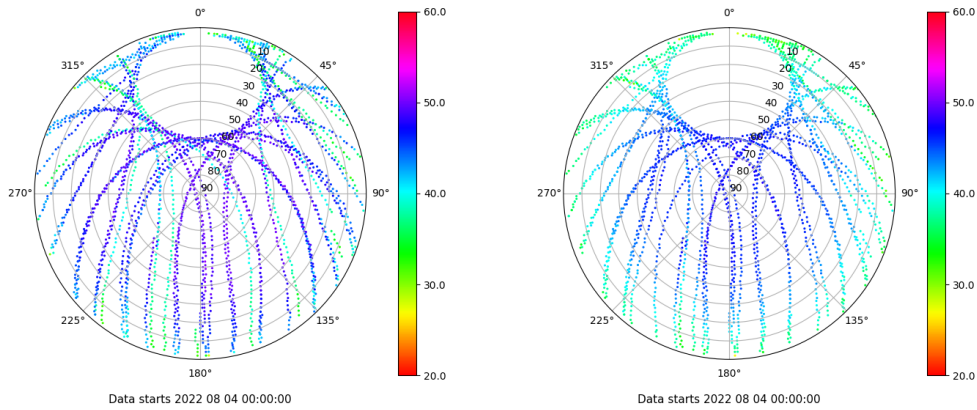
Skyplot for station RIO1. Signal to Noise S1C Data file RIO100ESP_R_2022216.xtr Skyplot for station RIO1. Signal to Noise S2P Data file RIO100ESP_R_2022216.xtr
