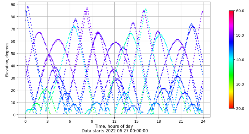
Time-elevation plot for station RIO1. Signal to Noise S1C Data file RIO100ESP_R_2022178.xtr
