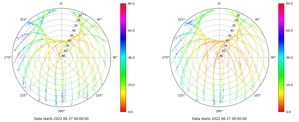
Skyplot for station RIO1. Parameter M1C Data file RIO100ESP_R_2022178.xtr Skyplot for station RIO1. Parameter M2P Data file RIO100ESP_R_2022178.xtr
