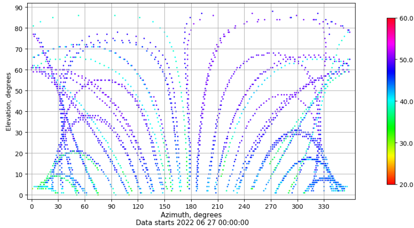
Azimuth-elevation plot for station RIO1. Signal to Noise S1C Data file RIO100ESP_R_2022178.xtr
