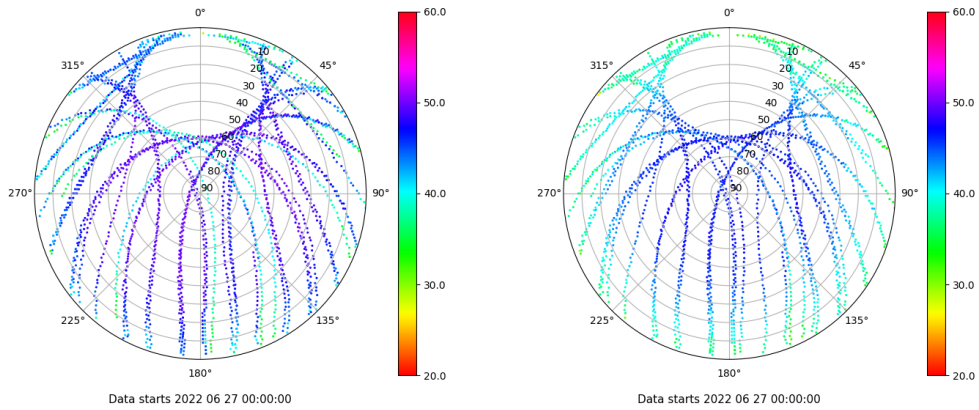
Skyplot for station RIO1. Signal to Noise S1C Data file RIO100ESP_R_2022178.xtr Skyplot for station RIO1. Signal to Noise S2P Data file RIO100ESP_R_2022178.xtr
