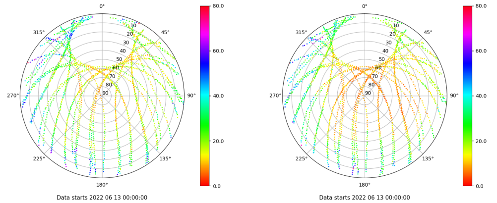
Skyplot for station RIO1. Parameter M1C Data file RIO100ESP_R_2022164.xtr Skyplot for station RIO1. Parameter M2P Data file RIO100ESP_R_2022164.xtr
