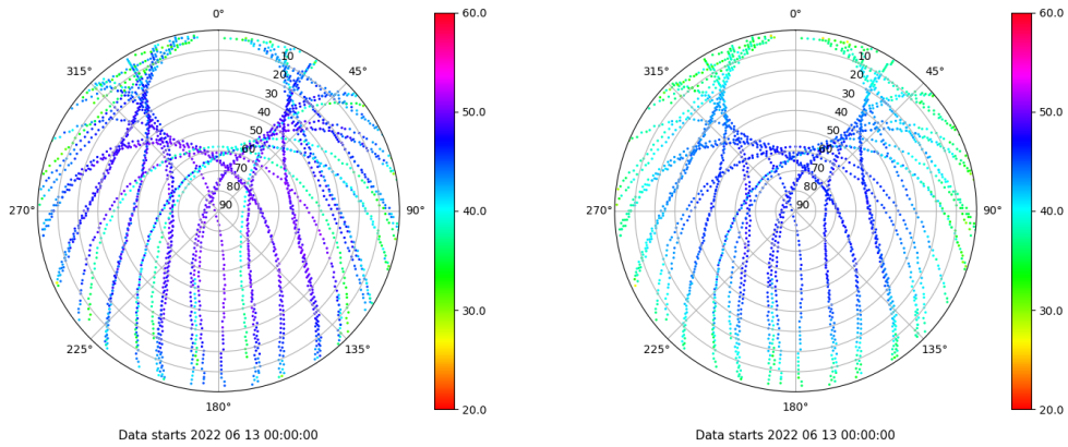
Skyplot for station RIO1. Signal to Noise S1C Data file RIO100ESP_R_2022164.xtr Skyplot for station RIO1. Signal to Noise S2P Data file RIO100ESP_R_2022164.xtr
