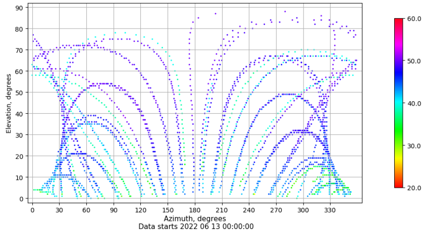
Azimuth-elevation plot for station RIO1. Signal to Noise S1C Data file RIO100ESP_R_2022164.xtr
