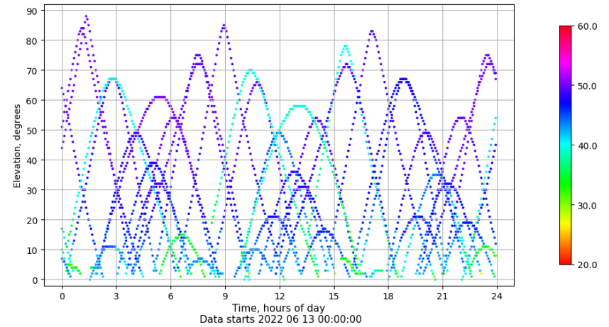
Time-elevation plot for station RIO1. Signal to Noise S1C Data file RIO100ESP_R_2022164.xtr
