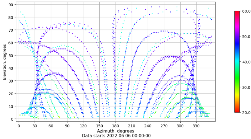
Azimuth-elevation plot for station RIO1. Signal to Noise S1C Data file RIO100ESP_R_2022157.xtr
