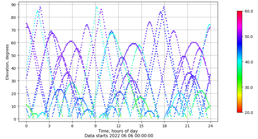
Time-elevation plot for station RIO1. Signal to Noise S1C Data file RIO100ESP_R_2022157.xtr
