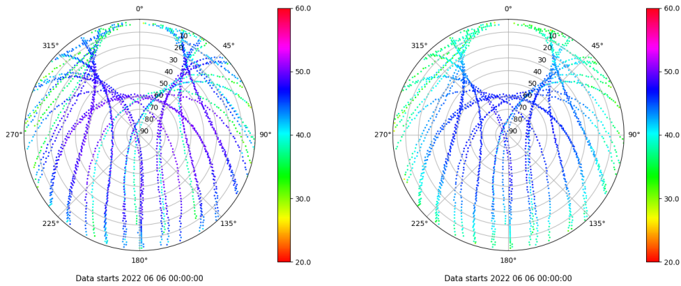
Skyplot for station RIO1. Signal to Noise S1C Data file RIO100ESP_R_2022157.xtr Skyplot for station RIO1. Signal to Noise S2P Data file RIO100ESP_R_2022157.xtr
