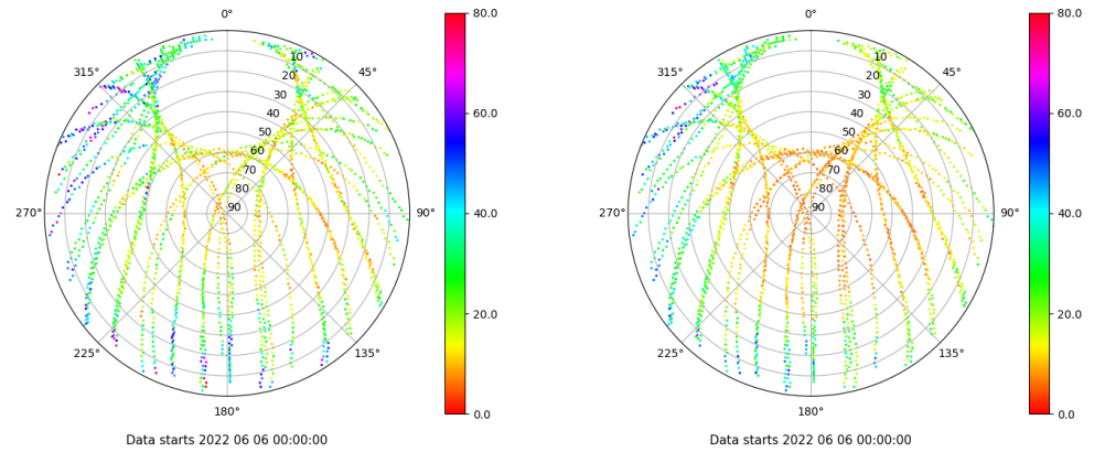
Skyplot for station RIO1. Parameter M1C Data file RIO100ESP_R_2022157.xtr Skyplot for station RIO1. Parameter M2P Data file RIO100ESP_R_2022157.xtr
