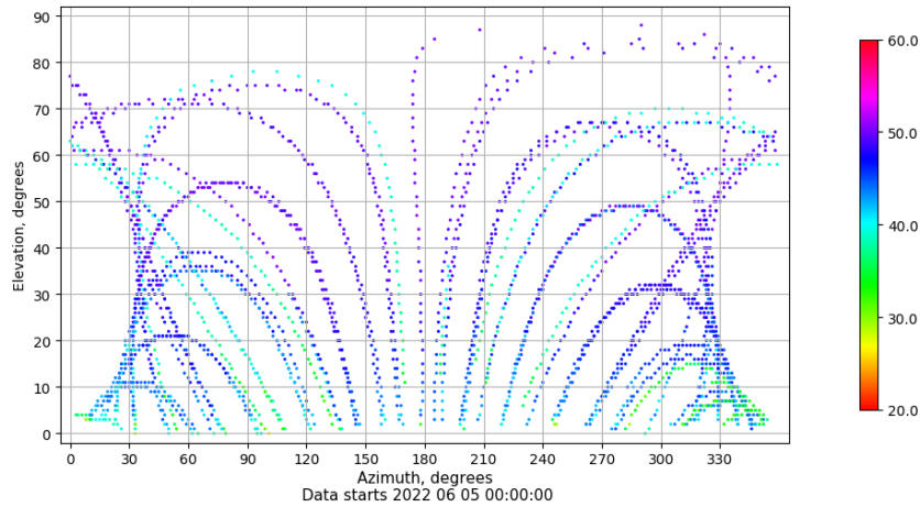
Azimuth-elevation plot for station RIO1. Signal to Noise S1C Data file RIO100ESP_R_2022156.xtr
