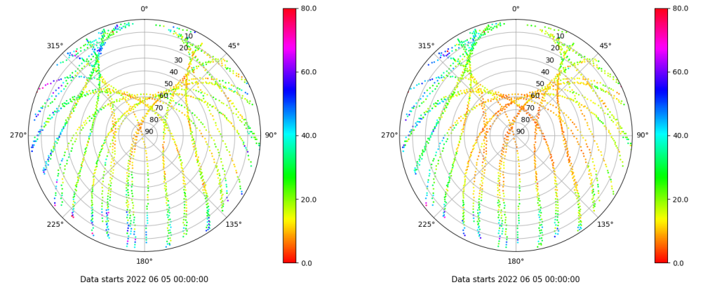
Skyplot for station RIO1. Parameter M1C Data file RIO100ESP_R_2022156.xtr Skyplot for station RIO1. Parameter M2P Data file RIO100ESP_R_2022156.xtr
