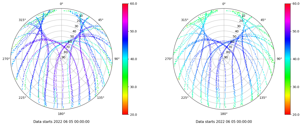
Skyplot for station RIO1. Signal to Noise S1C Data file RIO100ESP_R_2022156.xtr Skyplot for station RIO1. Signal to Noise S2P Data file RIO100ESP_R_2022156.xtr
