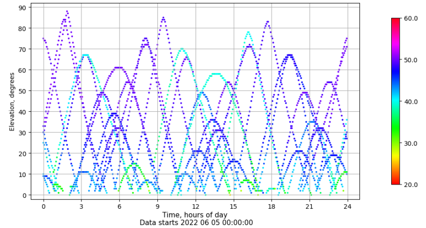
Time-elevation plot for station RIO1. Signal to Noise S1C Data file RIO100ESP_R_2022156.xtr
