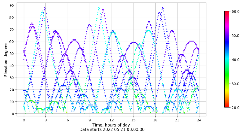
Time-elevation plot for station RIO1. Signal to Noise S1C Data file RIO100ESP_R_2022141.xtr
