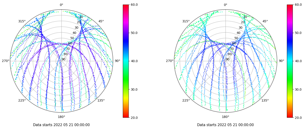
Skyplot for station RIO1. Signal to Noise S1C Data file RIO100ESP_R_2022141.xtr Skyplot for station RIO1. Signal to Noise S2P Data file RIO100ESP_R_2022141.xtr
