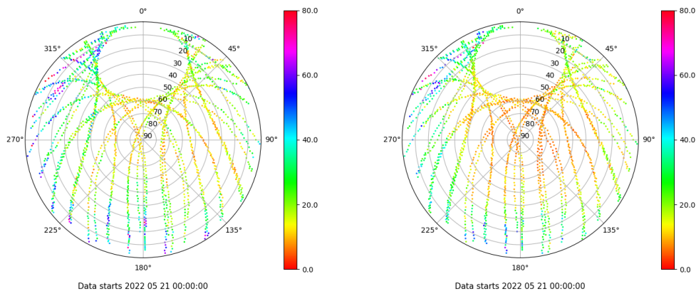
Skyplot for station RIO1. Parameter M1C Data file RIO100ESP_R_2022141.xtr Skyplot for station RIO1. Parameter M2P Data file RIO100ESP_R_2022141.xtr
