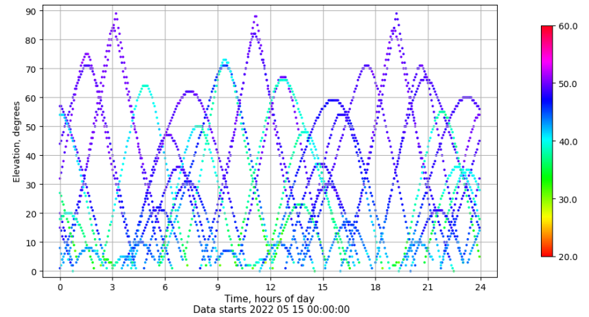
Time-elevation plot for station RIO1. Signal to Noise S1C Data file RIO100ESP_R_2022135.xtr
