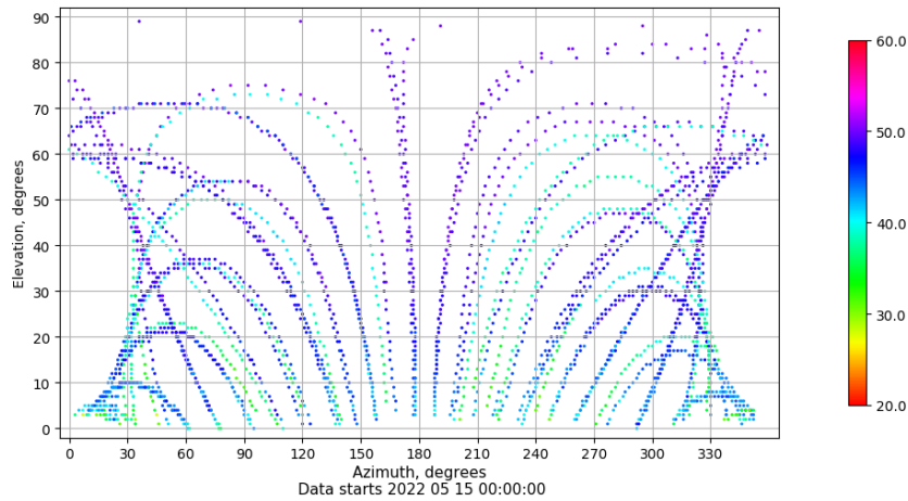
Azimuth-elevation plot for station RIO1. Signal to Noise S1C Data file RIO100ESP_R_2022135.xtr
