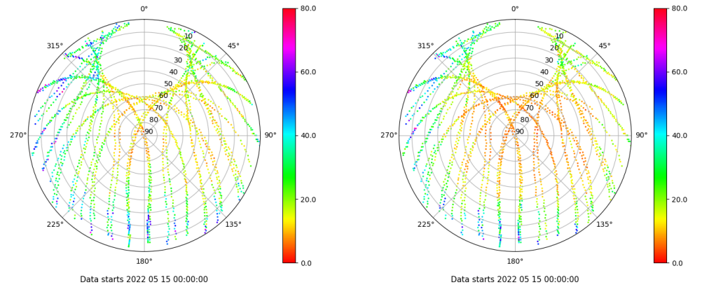
Skyplot for station RIO1. Parameter M1C Data file RIO100ESP_R_2022135.xtr Skyplot for station RIO1. Parameter M2P Data file RIO100ESP_R_2022135.xtr
