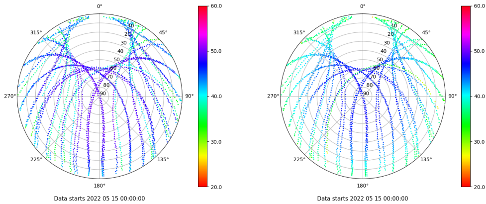
Skyplot for station RIO1. Signal to Noise S1C Data file RIO100ESP_R_2022135.xtr Skyplot for station RIO1. Signal to Noise S2P Data file RIO100ESP_R_2022135.xtr
