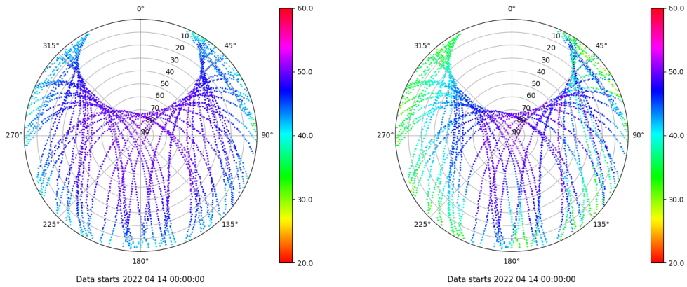
Skyplot for station RIO1. Signal to Noise S1C Data file RIO100ESP_R_2022104.xtr Skyplot for station RIO1. Signal to Noise S2W Data file RIO100ESP_R_2022104.xtr
