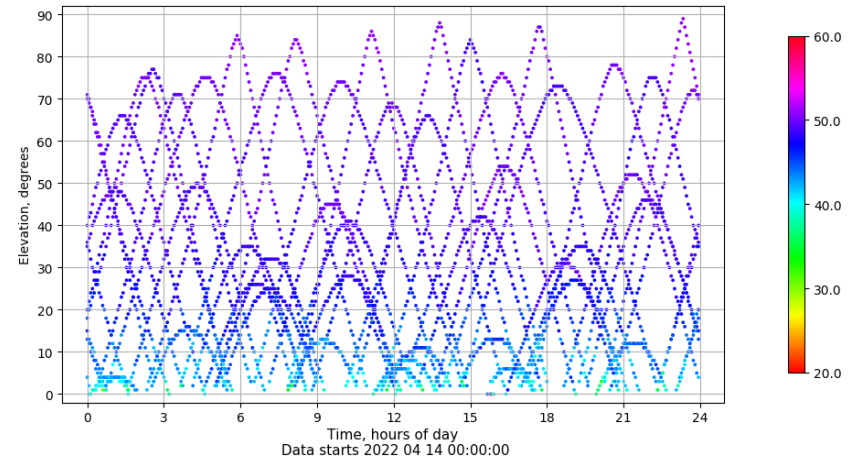
Time-elevation plot for station RIO1. Signal to Noise S1C Data file RIO100ESP_R_2022104.xtr
