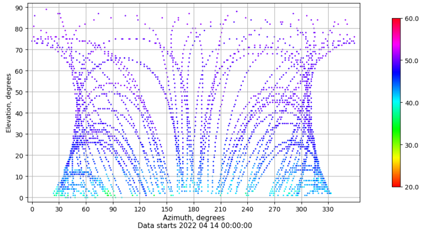
Azimuth-elevation plot for station RIO1. Signal to Noise S1C Data file RIO100ESP_R_2022104.xtr
