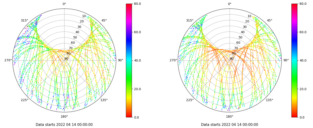
Skyplot for station RIO1. Parameter M1C Data file RIO100ESP_R_2022104.xtr Skyplot for station RIO1. Parameter M2W Data file RIO100ESP_R_2022104.xtr
