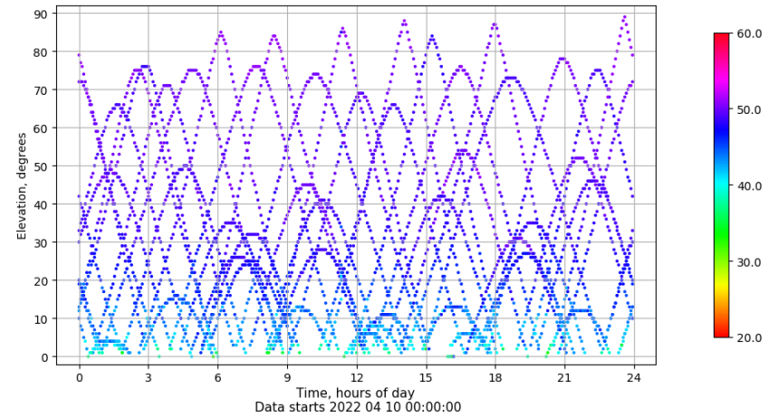
Time-elevation plot for station RIO1. Signal to Noise S1C Data file RIO100ESP_R_2022100.xtr
