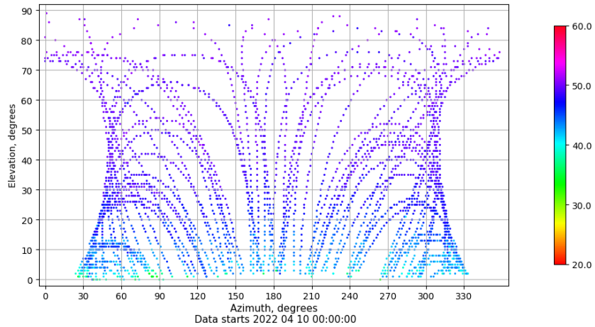
Azimuth-elevation plot for station RIO1. Signal to Noise S1C Data file RIO100ESP_R_2022100.xtr
