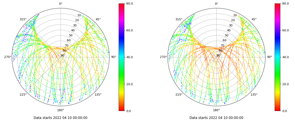
Skyplot for station RIO1. Parameter M1C Data file RIO100ESP_R_2022100.xtr Skyplot for station RIO1. Parameter M2W Data file RIO100ESP_R_2022100.xtr
