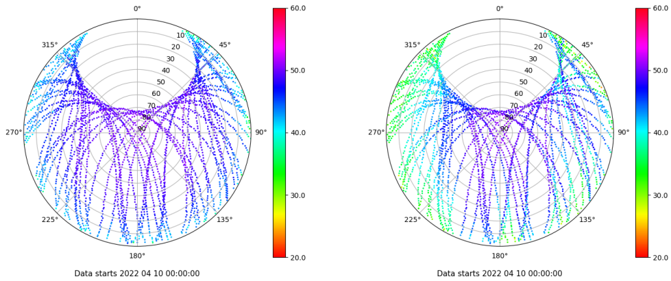
Skyplot for station RIO1. Signal to Noise S1C Data file RIO100ESP_R_2022100.xtr Skyplot for station RIO1. Signal to Noise S2W Data file RIO100ESP_R_2022100.xtr
