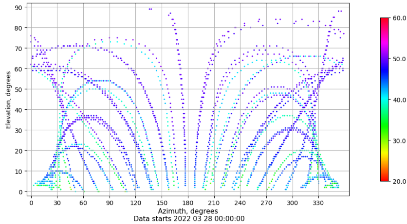
Azimuth-elevation plot for station RIO1. Signal to Noise S1C Data file RIO100ESP_R_2022087.xtr
