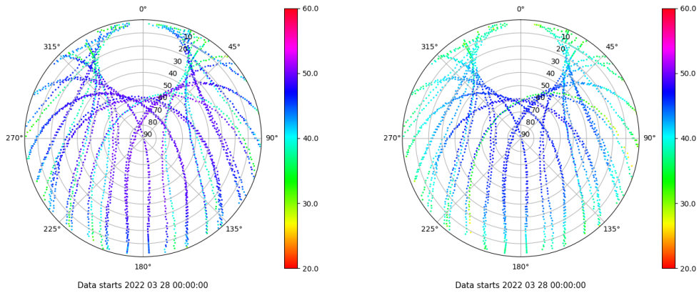
Skyplot for station RIO1. Signal to Noise S1C Data file RIO100ESP_R_2022087.xtr Skyplot for station RIO1. Signal to Noise S2P Data file RIO100ESP_R_2022087.xtr
