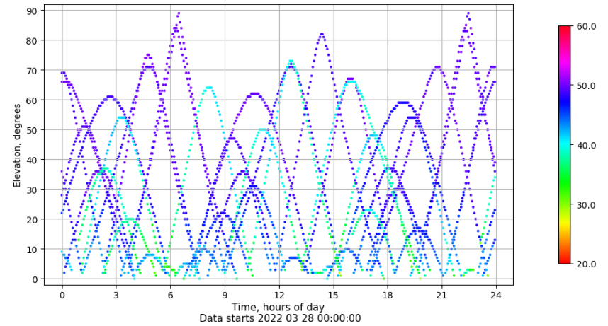
Time-elevation plot for station RIO1. Signal to Noise S1C Data file RIO100ESP_R_2022087.xtr
