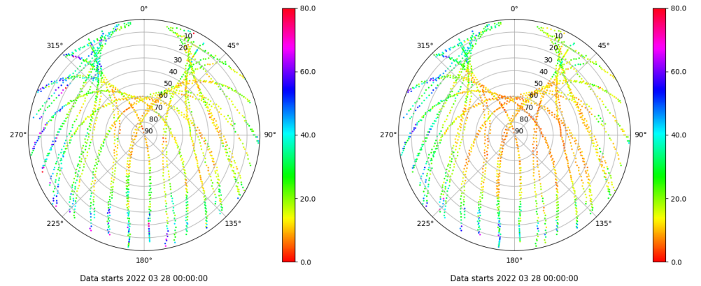
Skyplot for station RIO1. Parameter M1C Data file RIO100ESP_R_2022087.xtr Skyplot for station RIO1. Parameter M2P Data file RIO100ESP_R_2022087.xtr
