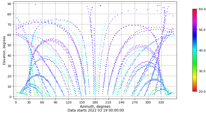
Azimuth-elevation plot for station RIO1. Signal to Noise S1C Data file RIO100ESP_R_2022078.xtr
