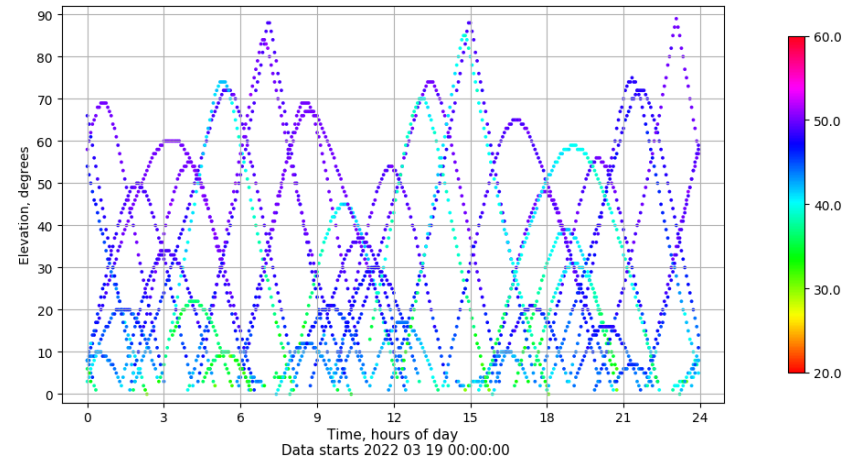
Time-elevation plot for station RIO1. Signal to Noise S1C Data file RIO100ESP_R_2022078.xtr
