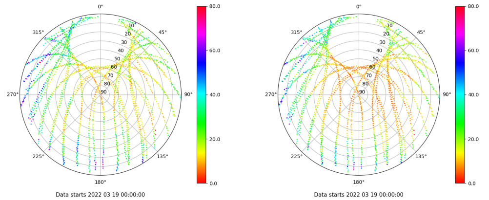
Skyplot for station RIO1. Parameter M1C Data file RIO100ESP_R_2022078.xtr Skyplot for station RIO1. Parameter M2P Data file RIO100ESP_R_2022078.xtr
