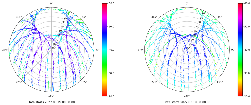
Skyplot for station RIO1. Signal to Noise S1C Data file RIO100ESP_R_2022078.xtr Skyplot for station RIO1. Signal to Noise S2P Data file RIO100ESP_R_2022078.xtr
