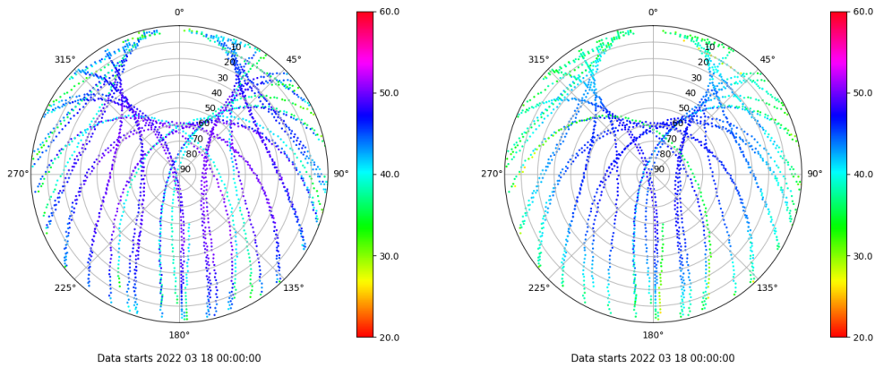
Skyplot for station RIO1. Signal to Noise S1C Data file RIO100ESP_R_2022077.xtr Skyplot for station RIO1. Signal to Noise S2P Data file RIO100ESP_R_2022077.xtr
