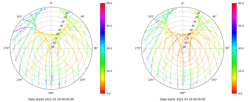
Skyplot for station RIO1. Parameter M1C Data file RIO100ESP_R_2022077.xtr Skyplot for station RIO1. Parameter M2P Data file RIO100ESP_R_2022077.xtr
