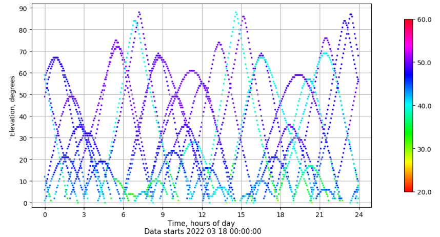
Time-elevation plot for station RIO1. Signal to Noise S1C Data file RIO100ESP_R_2022077.xtr
