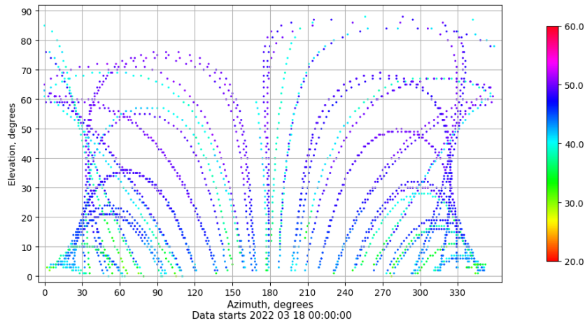
Azimuth-elevation plot for station RIO1. Signal to Noise S1C Data file RIO100ESP_R_2022077.xtr
