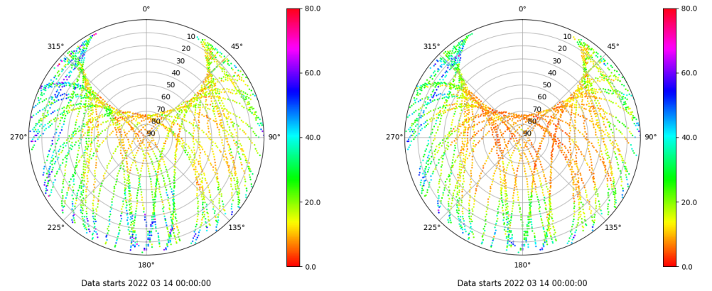
Skyplot for station RIO1. Parameter M1C Data file RIO100ESP_R_2022073.xtr Skyplot for station RIO1. Parameter M2W Data file RIO100ESP_R_2022073.xtr
