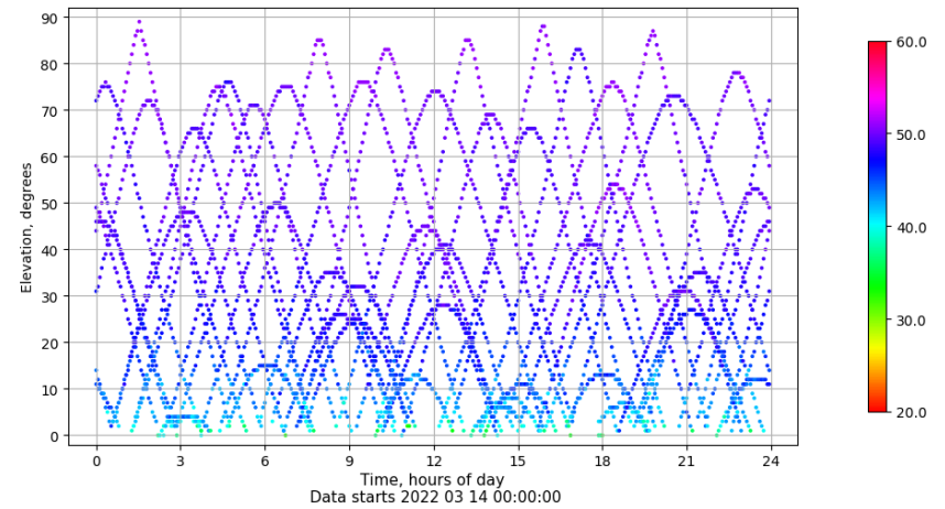
Time-elevation plot for station RIO1. Signal to Noise S1C Data file RIO100ESP_R_2022073.xtr
