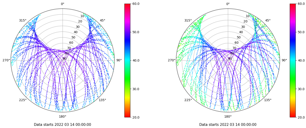
Skyplot for station RIO1. Signal to Noise S1C Data file RIO100ESP_R_2022073.xtr Skyplot for station RIO1. Signal to Noise S2W Data file RIO100ESP_R_2022073.xtr
