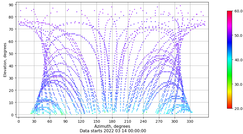
Azimuth-elevation plot for station RIO1. Signal to Noise S1C Data file RIO100ESP_R_2022073.xtr
