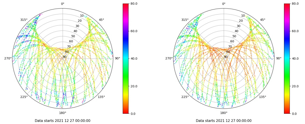
Skyplot for station RIO1. Parameter M1C Data file RIO100ESP_R_2021361.xtr Skyplot for station RIO1. Parameter M2W Data file RIO100ESP_R_2021361.xtr
