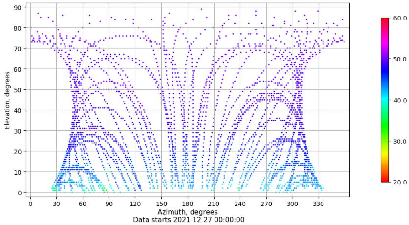
Azimuth-elevation plot for station RIO1. Signal to Noise S1C Data file RIO100ESP_R_2021361.xtr
