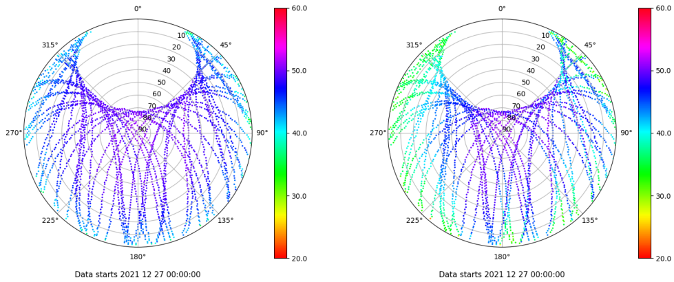
Skyplot for station RIO1. Signal to Noise S1C Data file RIO100ESP_R_2021361.xtr Skyplot for station RIO1. Signal to Noise S2W Data file RIO100ESP_R_2021361.xtr
