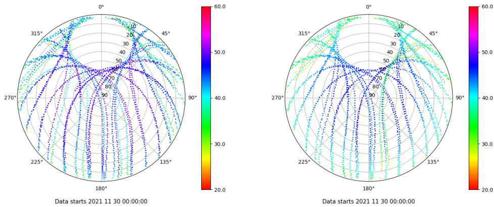
Skyplot for station RIO1. Signal to Noise S1C Data file RIO100ESP_R_2021334.xtr Skyplot for station RIO1. Signal to Noise S2P Data file RIO100ESP_R_2021334.xtr
