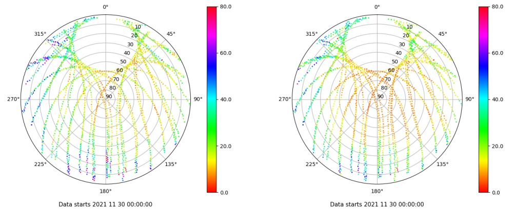
Skyplot for station RIO1. Parameter M1C Data file RIO100ESP_R_2021334.xtr Skyplot for station RIO1. Parameter M2P Data file RIO100ESP_R_2021334.xtr
