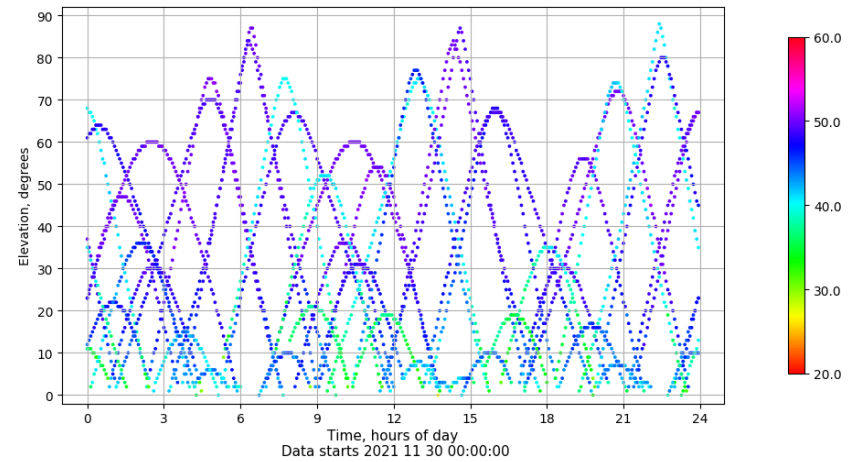
Time-elevation plot for station RIO1. Signal to Noise S1C Data file RIO100ESP_R_2021334.xtr
