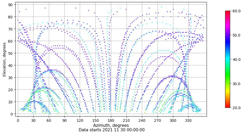
Azimuth-elevation plot for station RIO1. Signal to Noise S1C Data file RIO100ESP_R_2021334.xtr
