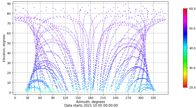
Azimuth-elevation plot for station RIO1. Signal to Noise S1C Data file RIO100ESP_R_2021278.xtr
