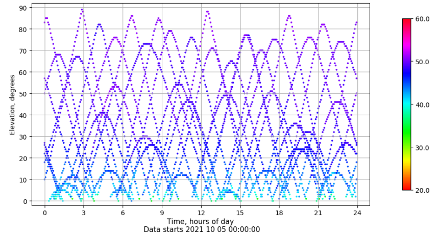
Time-elevation plot for station RIO1. Signal to Noise S1C Data file RIO100ESP_R_2021278.xtr
