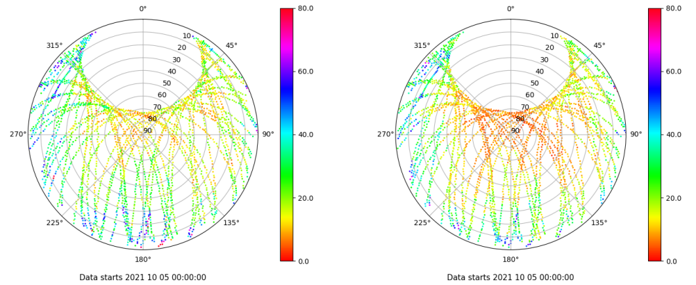
Skyplot for station RIO1. Parameter M1C Data file RIO100ESP_R_2021278.xtr Skyplot for station RIO1. Parameter M2W Data file RIO100ESP_R_2021278.xtr
