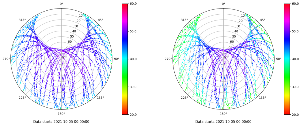
Skyplot for station RIO1. Signal to Noise S1C Data file RIO100ESP_R_2021278.xtr Skyplot for station RIO1. Signal to Noise S2W Data file RIO100ESP_R_2021278.xtr
